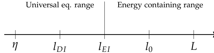
Figure 27: The different lengthscale's interplay in Kolmogorov's theory.
