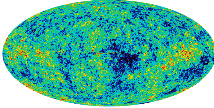
Figure 12: Behold! The Cosmic Microwave Background.
