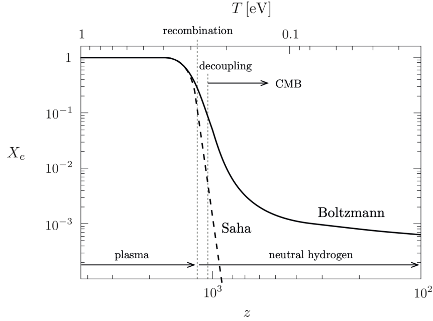
Figure 5: Free electron fraction as a function of redshift. The horizontal axis is reversed to replicate the natural flow of time from left to right. Credits: [1].
