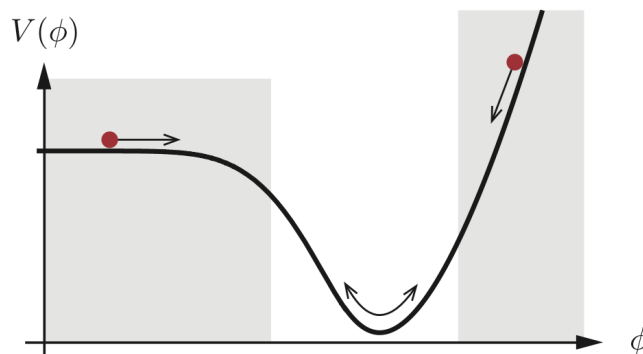
Figure 18: Example of a slow-roll potential as postulated by Linde, Albrecht, and Steinhardt. Inflation occurs in the shaded parts of the potential. Credits: [2].
