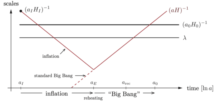
Figure 16: Scales of cosmological interest were larger than the Hubble radius until a \approx 10^{-5} (where today is at a(t_0) = 1 ). However, at very early times, before inflation operated, all scales of interest were smaller than the Hubble radius and therefore susceptible to microphysical processing. Notice the symmetry of the inflationary solution. Scales just entering the horizon today, 60 e -folds after the end of inflation, left the horizon 60 e -folds before the end of inflation. Credits: [2].
