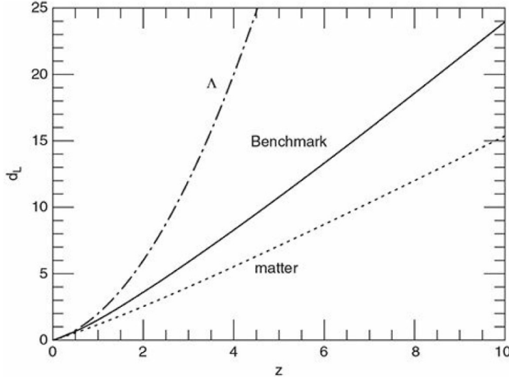
Figure 13: Luminosity distance of a standard candle with observed redshift z , in units of the Hubble distance, c/H_0 . The bold solid line gives the result for the Benchmark Model. For comparison, the dot-dash line indicates a flat, \Lambda -dominated Universe, and the dotted line a flat, matter-dominated Universe.
