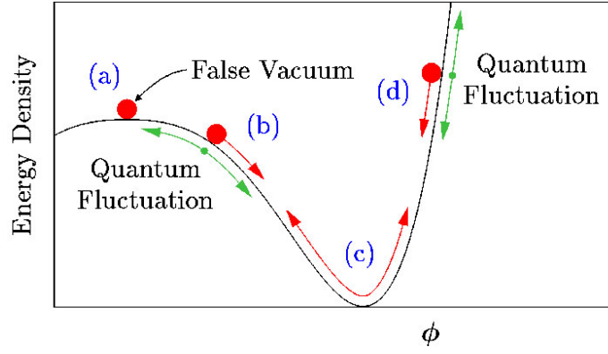
Figure 6.5: In simple inflationary models, the Universe at early times is dominated by the potential energy density of a scalar field, \phi . Red arrows show the classical motion of \phi . When \phi is near region (a), the energy density will remain nearly constant, \rho \approx \rho_f , even as the Universe expands. Moreover, cosmic expansion acts like a frictional drag, slowing the motion of \phi : Even near regions (b) and (d), \phi behaves more like a marble moving in a bowl of molasses, slowly creeping down the side of its potential, rather than like a marble sliding down the inside of a polished bowl. During this period of "slow roll," \rho remains nearly constant. Only after \phi has slid most of the way down its potential will it begin to oscillate around its minimum, as in region (c), ending inflation. Credits: this website .
