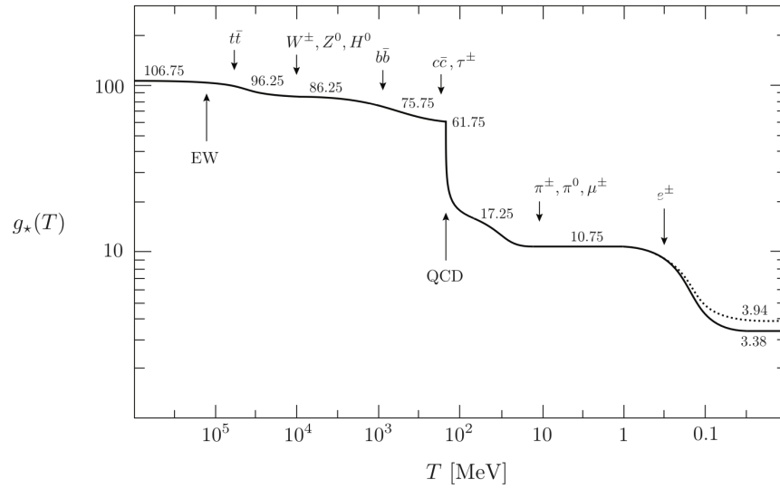
Figure 8: Evolution of relativistic degrees of freedom g_*(T) assuming the Standard Model particle content. The dotted line stands for the number of effective degrees of freedom in entropy g_{*S}(T) . Credits: [2].
