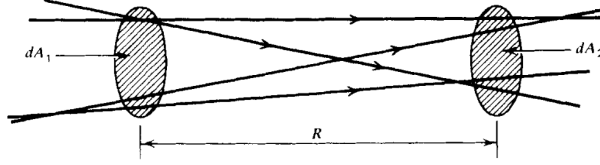
Figure 3.3: Geometrical construction for ray paths propagating in empty space. Credits: [12].
