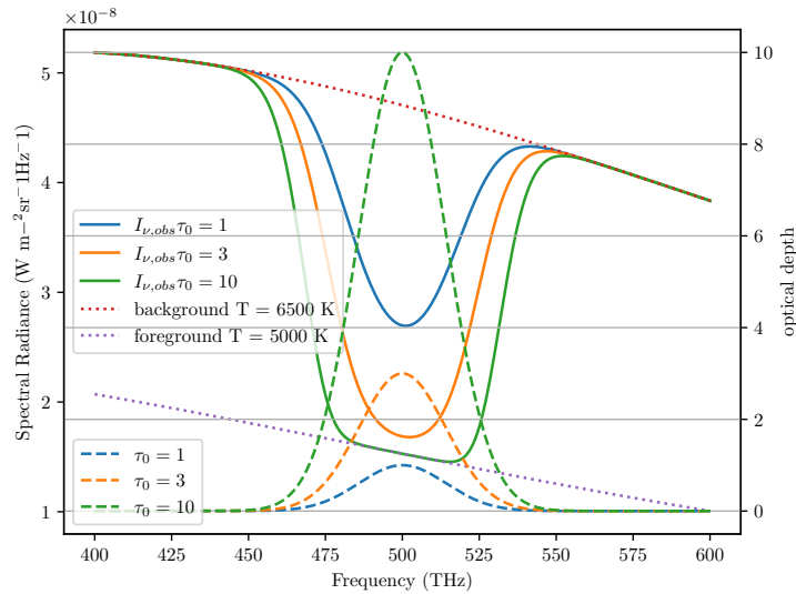
Figure 3.5: An example of absorption features formation for different temperatures and different values of \tau . Credits: Prof. Walter del Pozzo.
