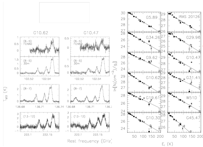
Figure 3.10: Rotational transitions of methyl-acetylene \text{CH}_3\text{C}_2\text{H} observed in molecular clumps associated with 12 ultracompact (UC) \text{H}_{\text{II}} regions. On the right, the associated Boltzmann diagrams. Credits: [6].
