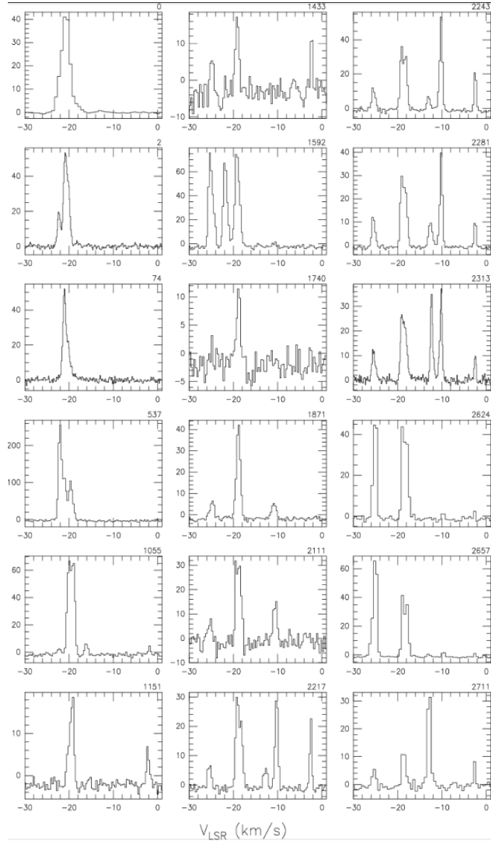
Figure 3.8: Variability of the H 2 O maser in the star forming region L1204-G.
