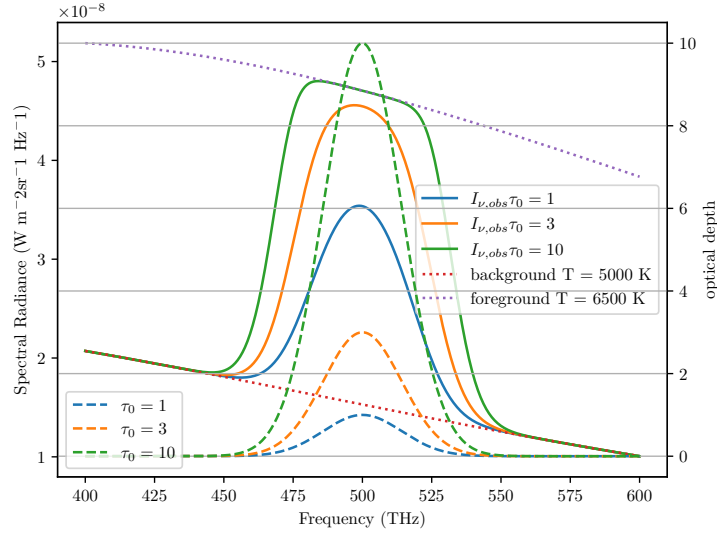
Figure 3.4: An example of emission features formation for different temperatures and different values of \tau . Credits: Prof. Walter del Pozzo.
