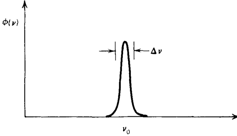
Figure 3.7: Line profile for a two levels atom. Credits: [12].
