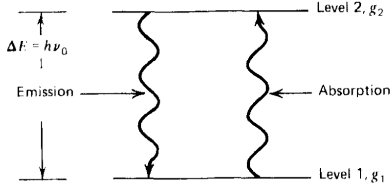
Figure 3.6: Photon emission and absorption in a two levels atom. Credits: [12].
