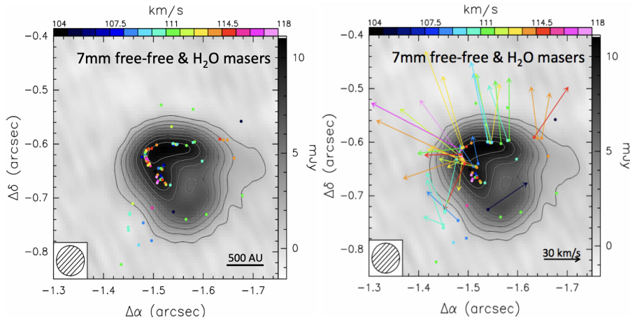
Figure 3.9: Analysis of 7 mm free-free radiation lines and H 2 O maser lines in a H II region. The panel on the right shows that the hypercompact H II region seems to be (generally) expanding. For more you can check [10].
