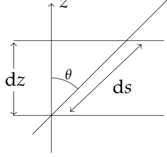
Figure 32: A ray path through a plane parallel atmosphere.
