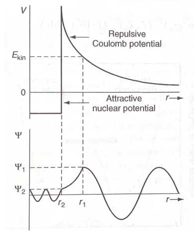
Figure 10: Illustration of the potential seen by a particle b when approaching a particle A with a kinetic energy E_{\text{kin}} and the corresponding wavefunction \Psi . Credits: [13].
