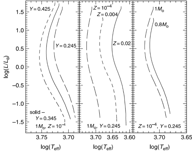
Figure 21: HRD location of Hayashi tracks for various assumptions about the chemical composition and the stellar mass. Credits: [16].
