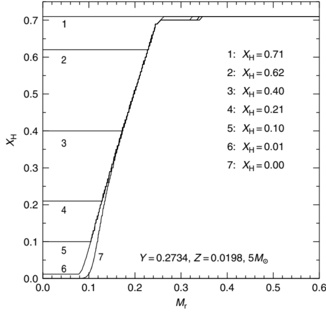
Figure 26: The chemical profile of Hydrogen in a 5M_{\odot} star at different stages. Credits:[16].
