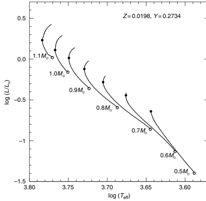
Figure 24: The HR diagram for LMS stars of different mass during the core H-burning phase. The solid dot marks the location of the turn off along each track. Credits: [16].
