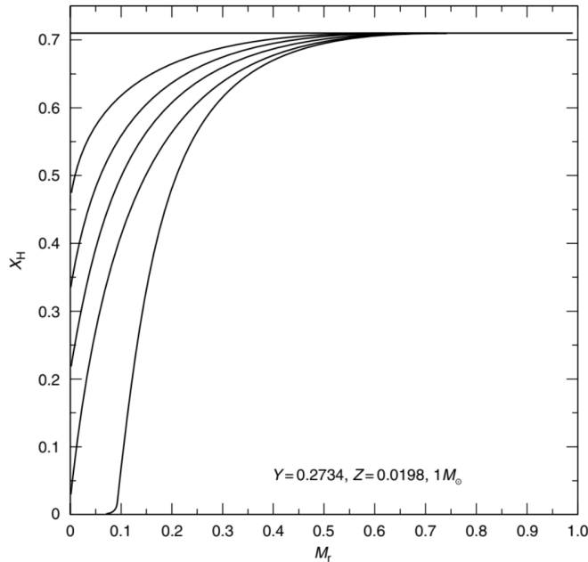
Figure 23: The chemical profile of Hydrogen in a 1M_{\odot} star at different stages during the core H-burning phase. Credits: [16].
