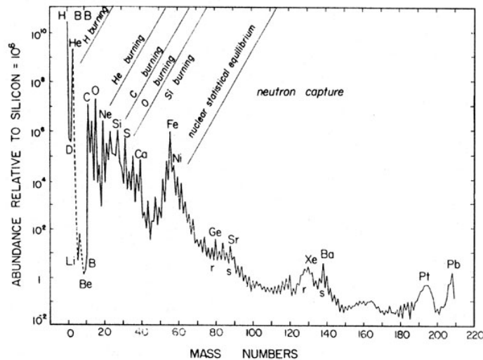
Figure 15: Numerical abundance of nuclides as observed in the Sun, normalized to 10^6 atoms of Silicon. Adapted from Cameron, 1920.
