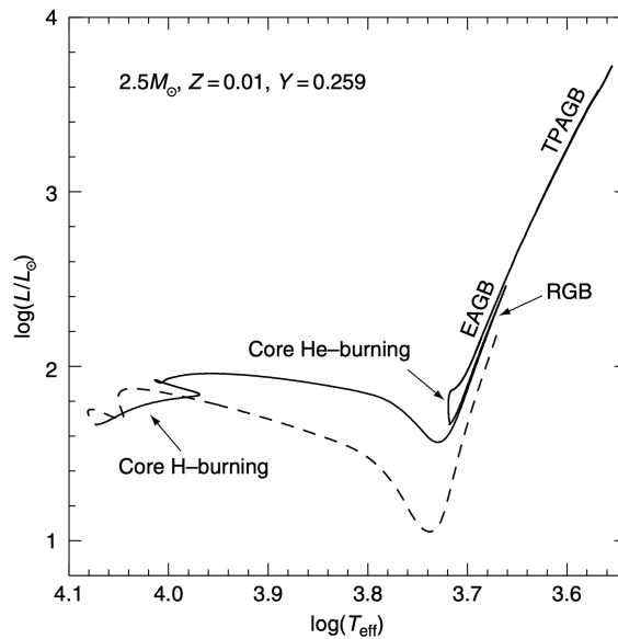
Figure 44: Evolutionary track of a 2.5M_{\odot} star from the PMS (dashed line) to the advanced TPAGB phase. Credits: [18].
