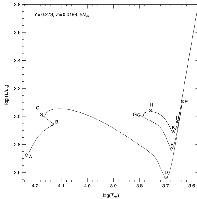
Figure 39: The evolutionary track of a 5M_{\odot} model during the Hydrogen and Helium burning phases. The different evolutionary stages discussed in the text are marked A-K. Credits: [18].
