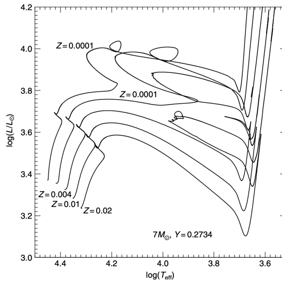
Figure 40: The HRD of evolutionary tracks of a 7M_{\odot} star for various values of the metallicity but with the same value for the initial He content. Credits: [18].
