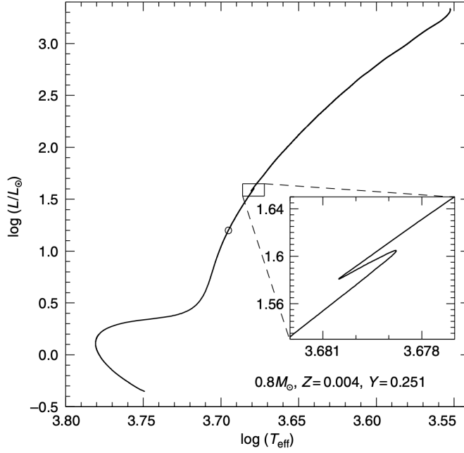
Figure 31: The HRD of the same 0.8M_{\odot} star from previous figures. The inset shows the trend of surface luminosity with the effective temperature when the H-burning shell crosses the chemical discontinuity produced by the first dredge up. The point along the evolutionary track corresponding to the first dredge up is marked with an open circle. Credits: [18].
