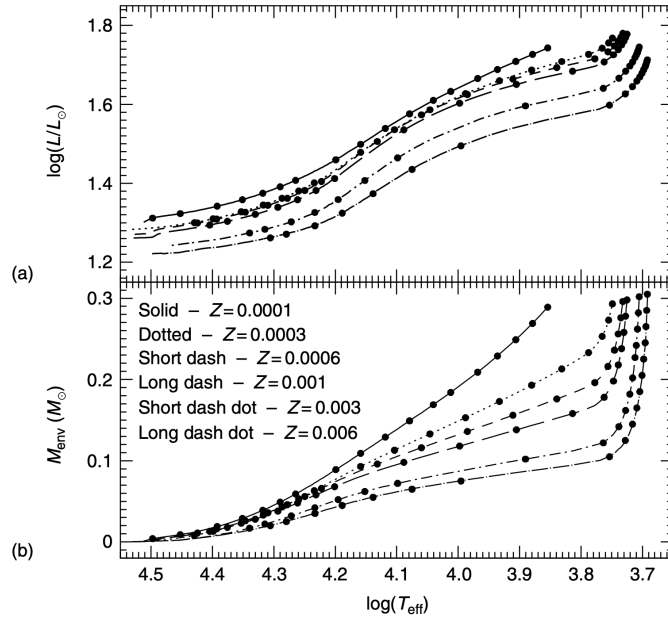
Figure 34: (a) The HR-diagram of the ZAHB for different values of the metallicity but the same RGB star progenitor, with M = 0.8 M_{\odot} . (b) The corresponding trend of the envelope mass as a function of their effective temperature. Solid dots in both (a) and (b) mark the location of selected ZAHB models. Credits: [18].
