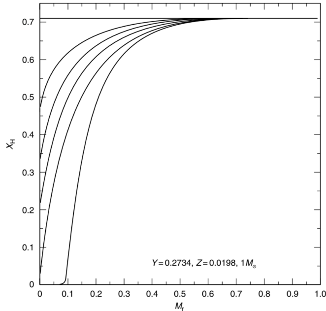
Figure 23: The chemical profile of Hydrogen in a 1M_{\odot} star at different stages during the core H-burning phase. Credits: [18].
