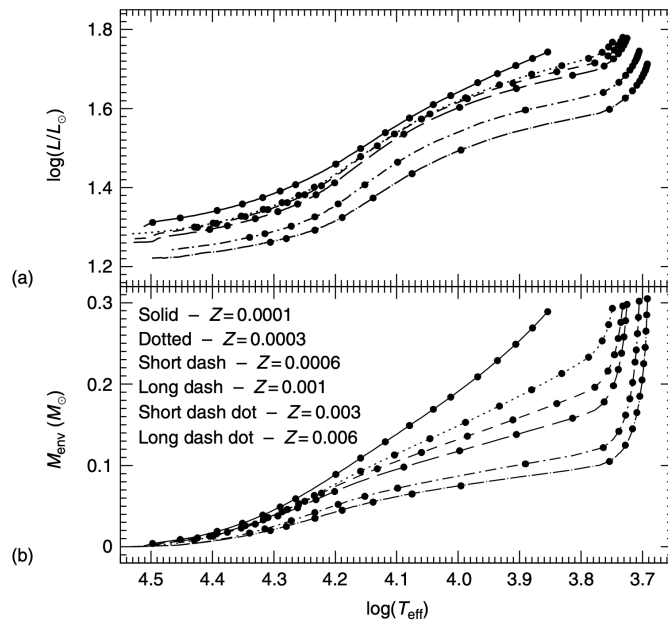
Figure 34: (a) The HR-diagram of the ZAHB for different values of the metallicity but the same RGB star progenitor, with M = 0.8M_{\odot} . (b) The corresponding trend of the envelope mass as a function of their effective temperature. Solid dots in both (a) and (b) mark the location of selected ZAHB models. Credits: [20].
