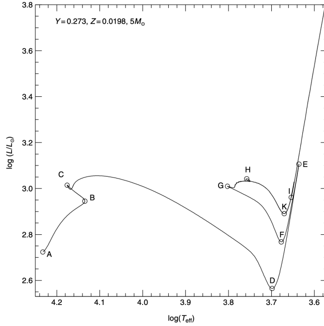
Figure 39: The evolutionary track of a 5M_{\odot} model during the Hydrogen and He-burning phases. The different evolutionary stages discussed in the text are marked A-K. Credits: [20].
