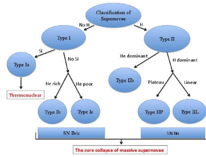
Figure 50: Supernova classification based on the presence of given elements features in the spectrum. Credits: [10].
