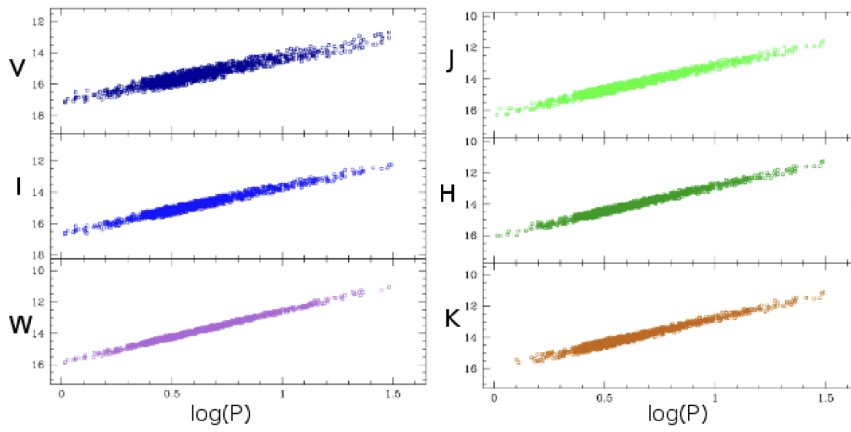
Figure 48: Dispersion of the P - L curve for various photometric bands. Note of the infrared K band and the W band (which is a band optimized for the purpose) are the narrower of the ones considered.
