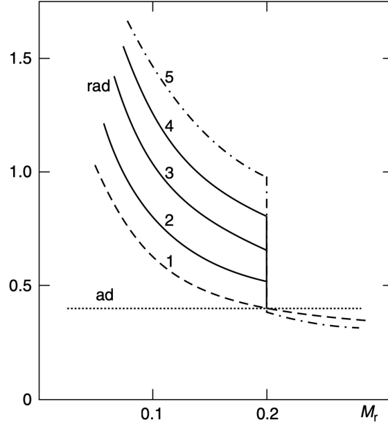
Figure 41: The growing discontinuity of the radiative temperature gradient at the boundary of the convective core for a core He-burning low-mass star. The numbers mark a time sequence (time is increasing going from stage 1 to stage 5). Credits: [20].
