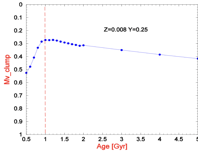
Figure 38: Magnitude in the Visual band of the red clump as a function of the age of the cluster. Note how only for ages higher than \sim 1 Gyr the clump luminosity is approximately independent on the age. Credits: Professor S. Degl'Innocenti and the PISA group.
