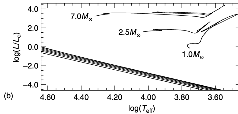
Figure 53: HRD location of WD evolutionary tracks for different values of the white dwarf's mass compared with previous evolutionary phases. Credits: [20].
