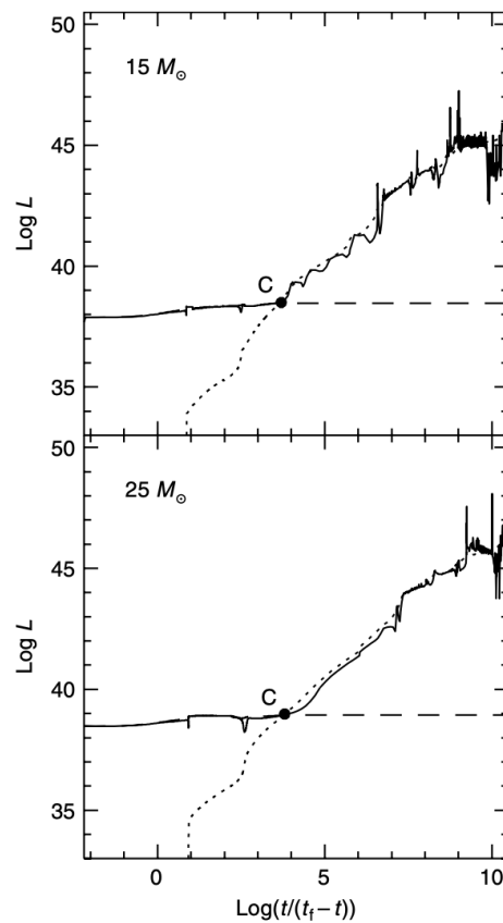
Figure 49: Behaviour with time of various luminosities (in \text{erg s}^{-1} ) for two massive stars: the dashed line corresponds to the surface luminosity, the solid one to the energy produced by the nuclear burning, while the dotted lines refers to the neutrinos' energy. The solid dot marks the ignition of the core C-burning. Credits: [20].
