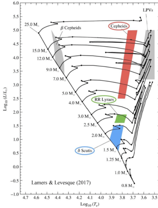
Figure 47: Location in the HRD of various pulsating stars. Cepheids, RR-Lyrae and \delta -Scuti stars are located in a nearly vertical instability strip. The Long Period Variables are outside the strip.
