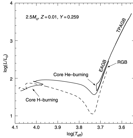
Figure 44: Evolutionary track of a 2.5M_{\odot} star from the PMS (dashed line) to the advanced TPAGB phase. Credits: [20].
