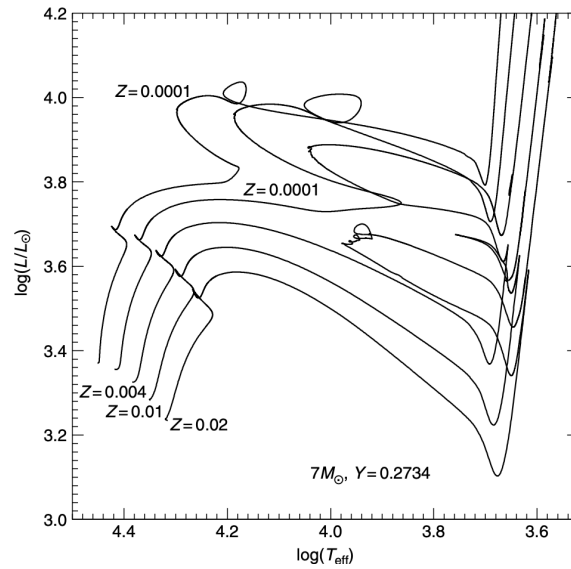
Figure 40: The HRD of evolutionary tracks of a 7M_{\odot} star for various values of the metallicity but with the same value for the initial He content. Credits: [20].
