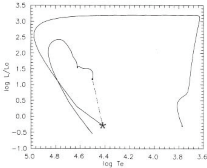
Figure 36: Evolutive trajectory for a "Hot Flasher" model. The * marks the Helium Flash ignition and the dashed line connects said point with the first quiescent burning model for Helium in the core. The following evolution in the quiescent Helium burning phase until the final cooling and settling into a CO WD is also shown. Credits: Unknown.
