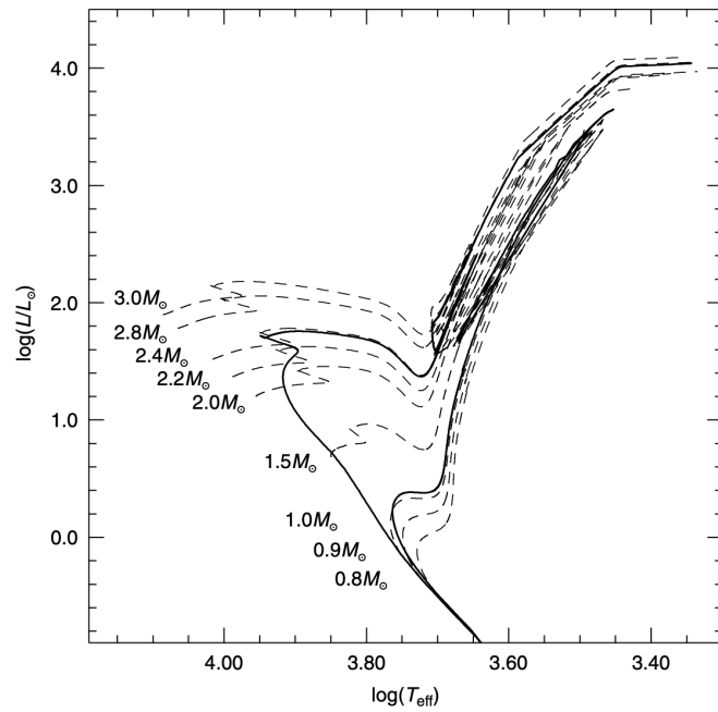
Figure 33: HRD of selected stellar evolutionary tracks (dashed lines) with the same initial solar chemical composition and the labelled masses. The heavy solid lines display two isochrones for the same chemical composition and ages of 600 Myr (the brighter sequence) and 10 Gyr. Credits: [20].
