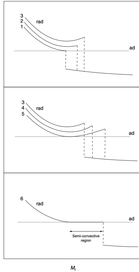
Figure 42: Qualitative behaviour of the radiative temperature gradient near the boundary of the convective core during the core He-burning phase, showing the time sequence of the events which result in the appearance of a semi-convective region. The numbers mark a time sequence (time is increasing going from stage 1 to stage 6). Credits:[20].
