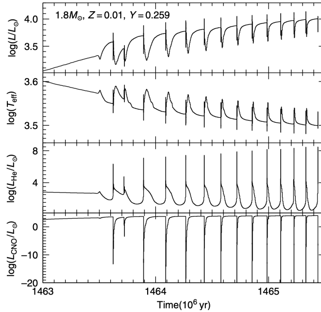
Figure 46: Evolution with time of the effective temperature, surface luminosity, luminosity associated with the He-burning in the shell, and the luminosity produced through the CNO cycle in the H-burning shell, during the first series of thermal pulses of a 1.8M_{\odot} star. Credits: [20].
