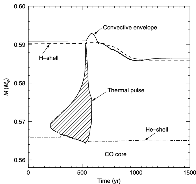
Figure 45: Evolution with time of part of the internal structure of a 2M_{\odot} star with Z = 0.015 and Y = 0.275 , during the tenth thermal pulse; the locations of the H-burning shell, the He-burning shell and the base of the convective envelope are shown. The origin of the time coordinate has been arbitrarily shifted. The dashed zone shows the development of the convective region during the thermal pulse. Notice the occurrence of the third dredge up about 200 yr after the onset of the thermal pulse. Credits: [20] and O. Straniero.
