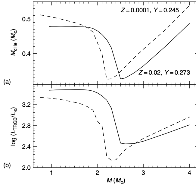
Figure 32: (a) The behaviour of the mass of the Helium core and (b) of the surface luminosity at the onset of He-burning as a function of the stellar mass for two selected initial chemical compositions. Credits: [20].
