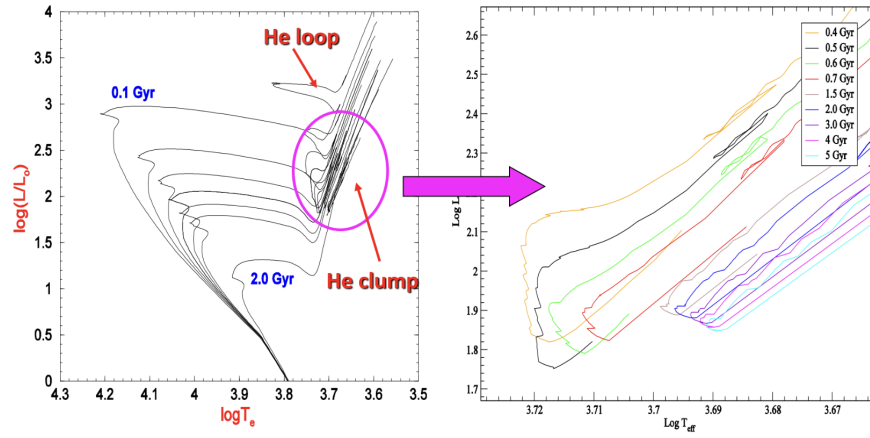
Figure 37: On the left cartoon, theoretical isochrones for stellar clusters displaying the whole MS, SGB and RGB phases. The Helium clump and the Helium loop are also visible. On the right cartoon, zoom on the red clump, highlighting its dependence on age. Credits: Professor S. Degl'Innocenti and the PISA group.
