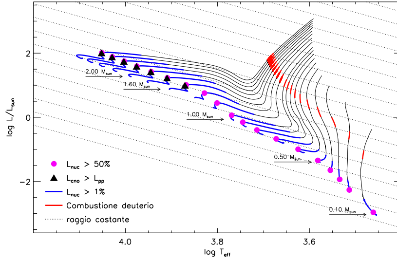
Figure 20: Evolution of different mass stars along the protostar and PMS stage. The red segments indicate the stage during which Deuterium is burned, while the blue segments indicate the stage where the luminosity generated by nuclear reactions is over 1%.
