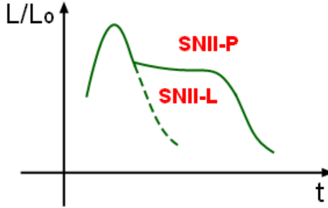
Figure 51: Morphological difference in the lightcurve between a Type IIL and a Type IIP SN. Credits: Wikipedia.
