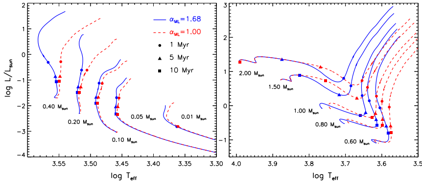
Figure 22: Effect of convection on the evolution of a star along the Hayashi track and further. Note how the great divergences introduced by convection early on are quickly smoothened away as the star progresses towards MS.
