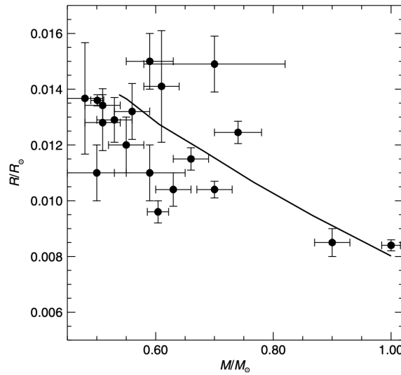
Figure 52: Comparison of the theoretical mass-radius relationship predicted by theoretical models with observations. With more recent data (perhaps those of the GAIA DR3) you could probably do better than this. But still- Credits: [20].
