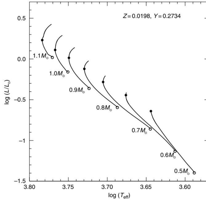
Figure 24: The HR diagram for LMS stars of different mass during the core H-burning phase. The solid dot marks the location of the turn off along each track. Credits: [20].
