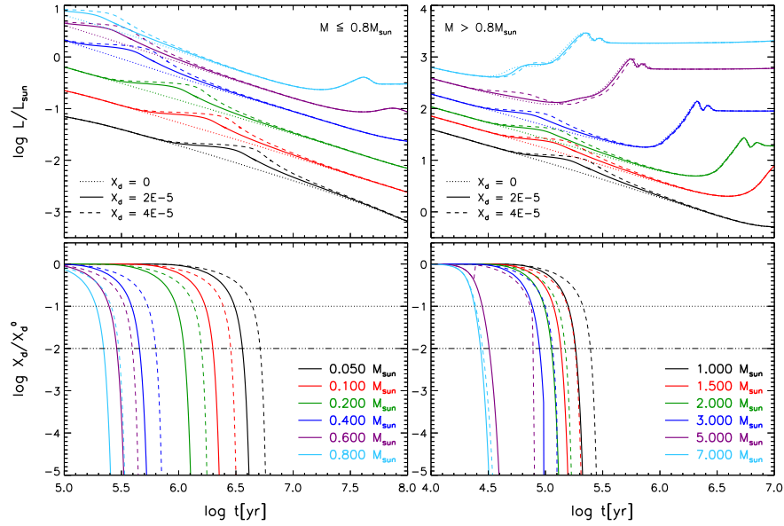
Figure 20: In the upper cartoons the evolution of luminosity over time for different initial abundances of Deuterium for masses M \leq 0.8 M_{\odot} (on the left), and M \geq 0.8 M_{\odot} (on the right). In the lower cartoons, the evolution of Deuterium abundance over time for different masses.
