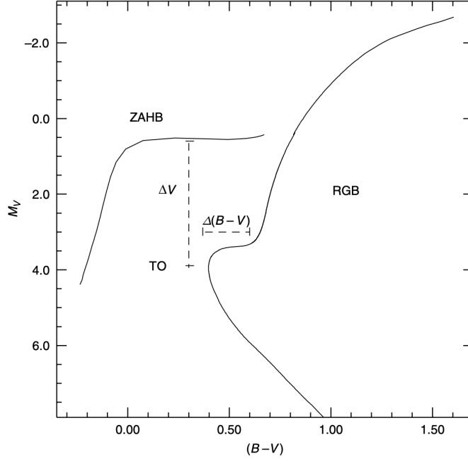
Figure 36: Graphical representation of the \Delta V (vertical) and \Delta(B - V) (horizontal) age indicators for old SSPs.
