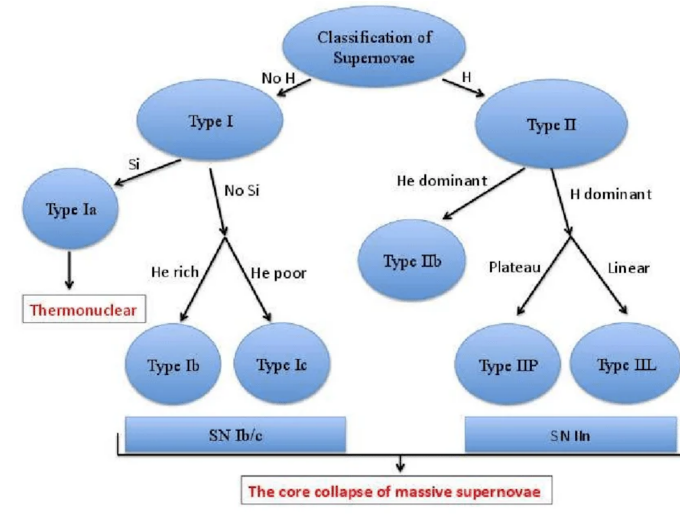
Figure 51: Supernova classification based on the presence of given elements features in the spectrum. Credits: [10].
