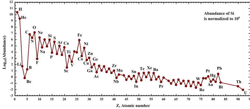
Figure 6: Universal curve of abundances, normalized on the relative abundance of Silicon. It represents the average value in the galactic disk of chemical abundances in stars. Credits: Wikipedia, but potentially [1].
