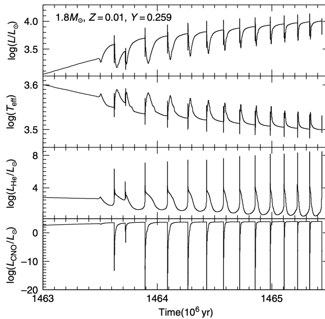
Figure 46: Evolution with time of the effective temperature, surface luminosity, luminosity associated with the He-burning in the shell, and the luminosity produced through the CNO cycle in the H-burning shell, during the first series of thermal pulses of a 1.8M_{\odot} star. Credits: [20].
