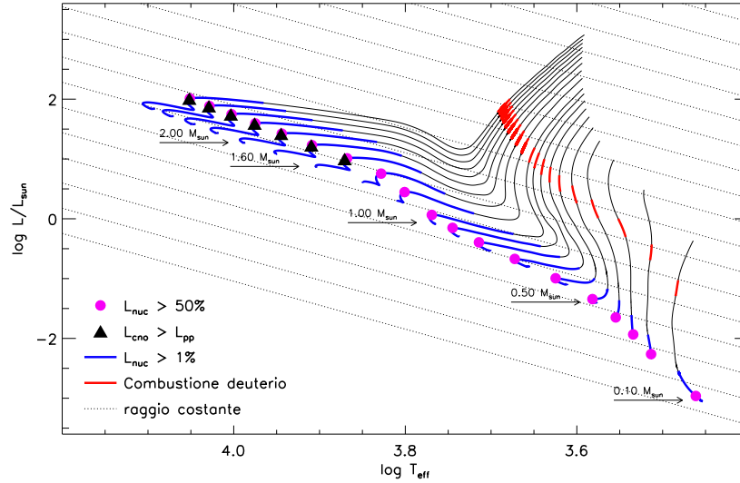
Figure 20: Evolution of different mass stars along the protostar and PMS stage. The red segments indicate the stage during which Deuterium is burned, while the blue segments indicate the stage where the luminosity generated by nuclear reactions is over 1%.
