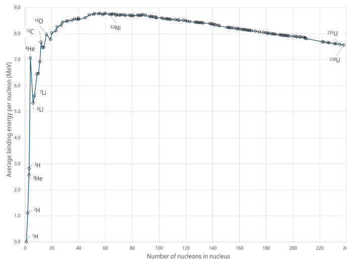
Figure 9: Binding energy per nucleon for a selection of nuclides. The nuclide with the highest value, ^{62}\text{Ni} , is noted.
