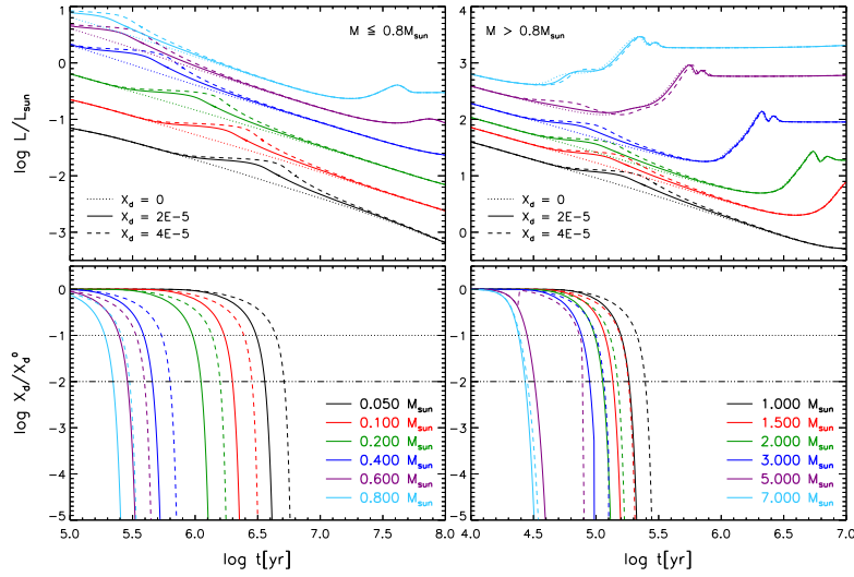
Figure 19: In the upper cartoons the evolution of luminosity over time for different initial abundances of Deuterium for masses M \leq 0.8 M_{\odot} (on the left), and M \geq 0.8 M_{\odot} (on the right). In the lower cartoons, the evolution of Deuterium abundance over time for different masses.
