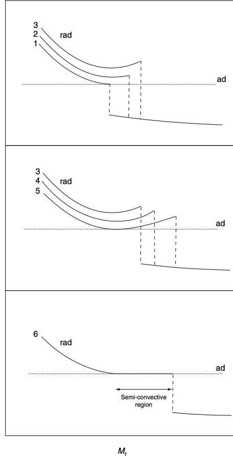
Figure 43: Qualitative behaviour of the radiative temperature gradient near the boundary of the convective core during the core He-burning phase, showing the time sequence of the events which result in the appearance of a semi-convective region. The numbers mark a time sequence (time is increasing going from stage 1 to stage 6). Credits:[21].
