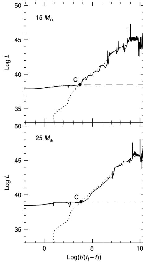
Figure 50: Behaviour with time of various luminosities (in \text{erg s}^{-1} ) for two massive stars: the dashed line corresponds to the surface luminosity, the solid one to the energy produced by the nuclear burning, while the dotted lines refers to the neutrinos' energy. The solid dot marks the ignition of the core C-burning. Credits: [21].
