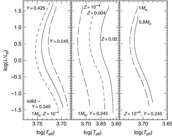
Figure 22: HRD location of Hayashi tracks for various assumptions about the chemical composition and the stellar mass. Credits: [21].
