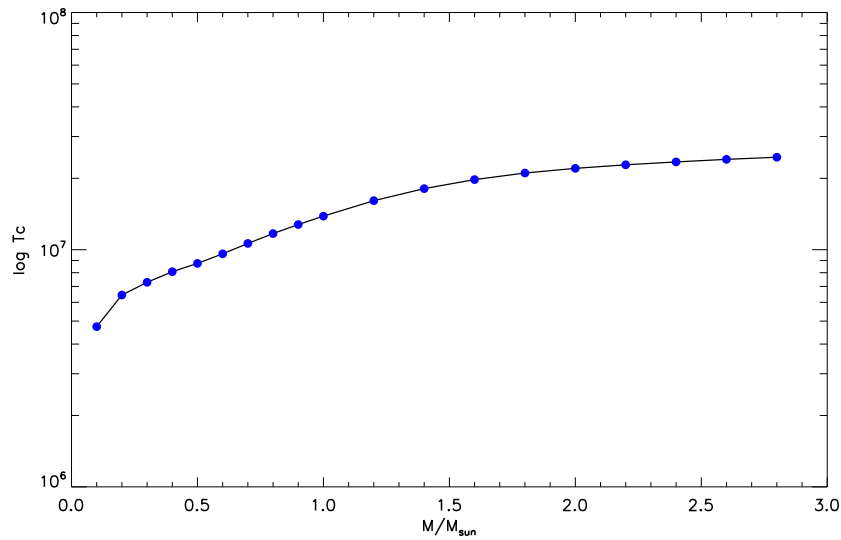
Figure 28: Curve representing how the central temperature of star varies depending on the star mass. Note how the slope of the curve changes around 1 - 1.2M_{\odot} , where the transition between LMS and UMS is.
