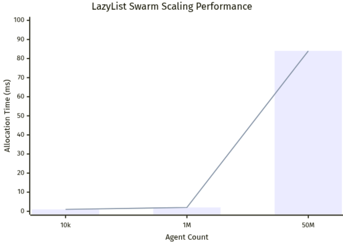
Figure 1: Computational scaling and allocation performance of the LazyList swarm sizing model.
