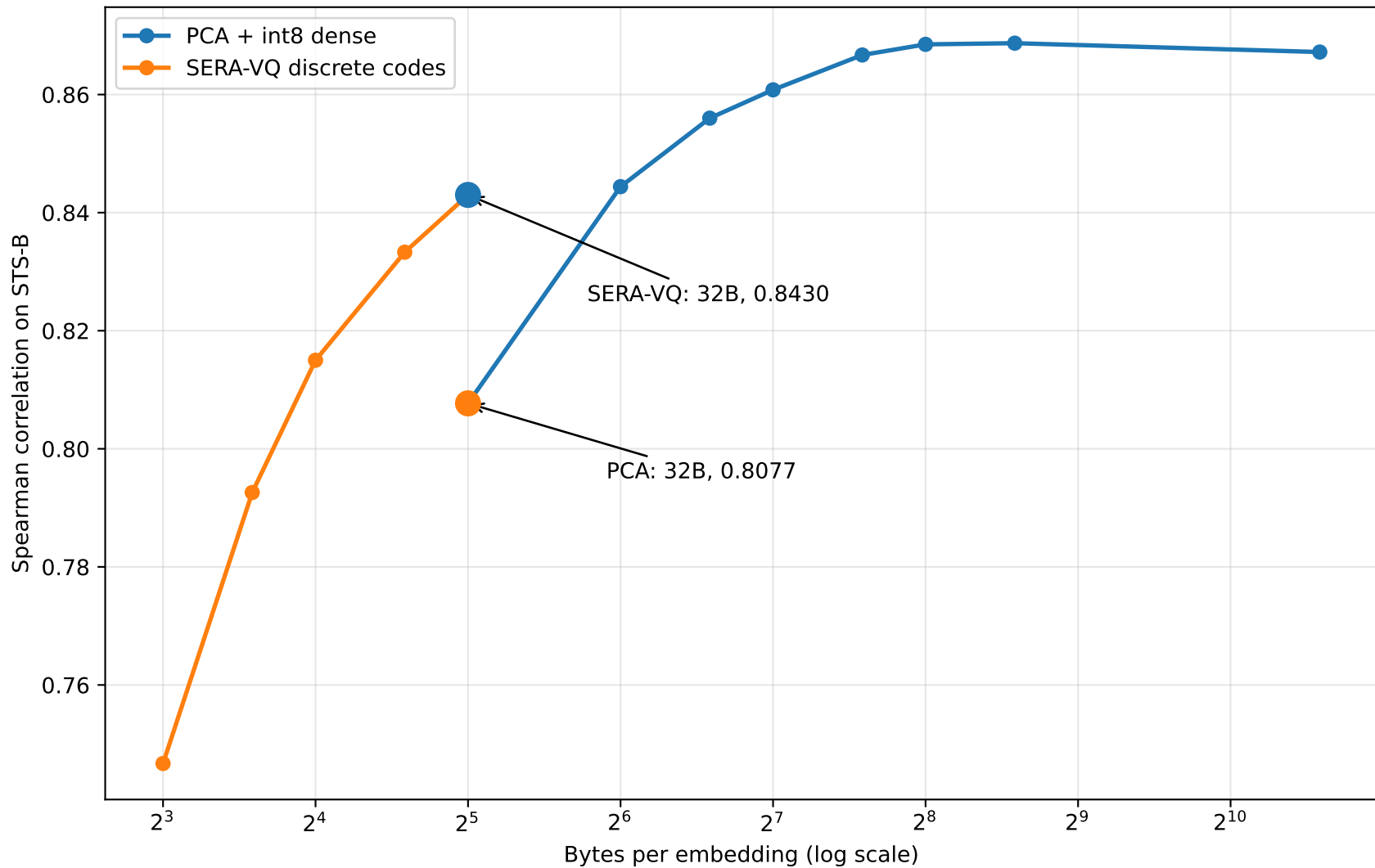
Discrete Codes Dominate Dense PCA at Low Memory Budgets
