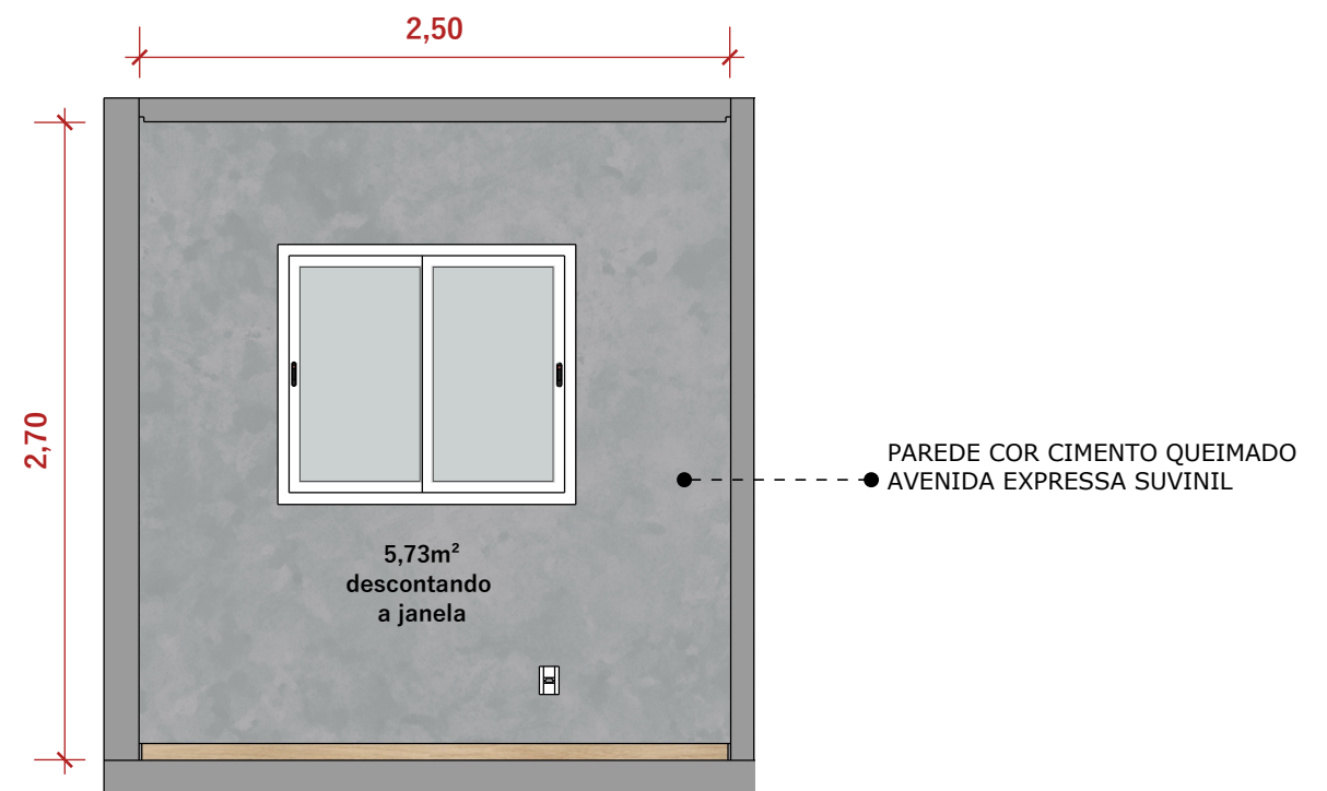
VISTA 2 - HOME OFFICE ESC 1:35
