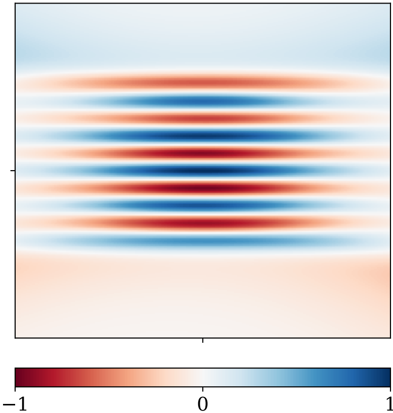
approximation PINN (Epoch 100)
