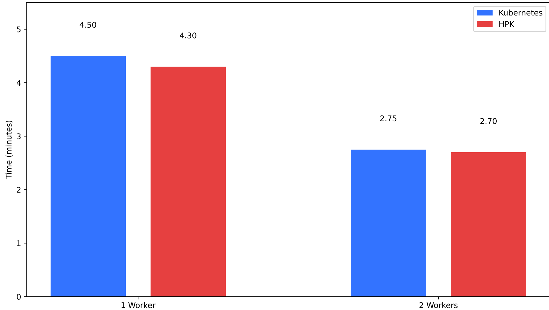
Distributed ML Training: Kubernetes vs HPK (GPU)
