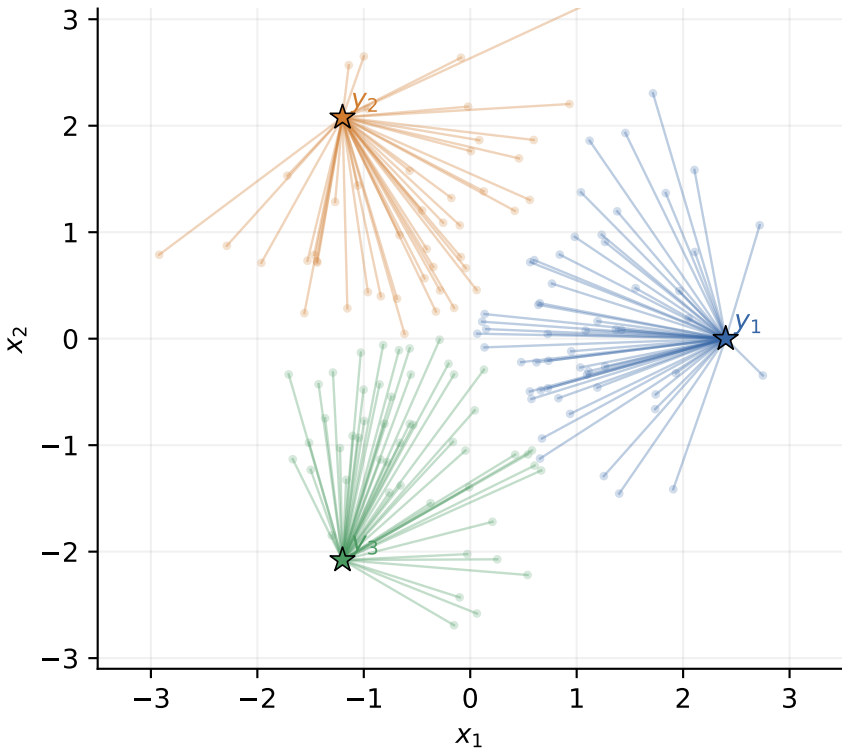
semi-discrete OT rays
