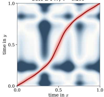
soft-DTW, \epsilon = 0.200
