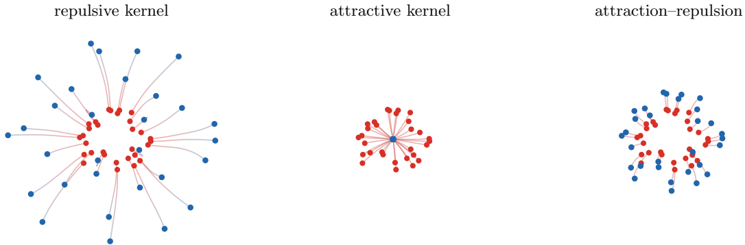
Figure 53: Interaction-energy particle flows for three choices of k . A positive Gaussian kernel k(x, y) = \exp(-\|x - y\|^2 / (2\sigma^2)) produces short-range repulsion under Wasserstein descent; changing its sign produces attraction and collapse; adding a quadratic long-range attraction to the repulsive kernel yields a balanced attraction–repulsion dynamics. In all cases the particles follow the coupled ODE structure of (143).
