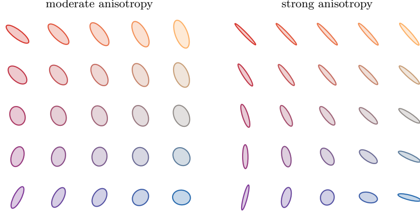
Figure 43: Bures–Wasserstein barycenters of centered Gaussian covariance matrices. Each panel shows a 5 \times 5 grid of barycenter ellipses for four corner covariances, without separate input panels: the corner ellipses are the four input covariances themselves. The right grid uses more anisotropic inputs, making the nonlinear rotation and scaling of covariance barycenters more visible.
