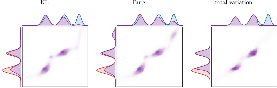
Figure 37: Effect of the marginal divergence in unbalanced entropic OT. The geometric cost, entropic plan regularization \varepsilon , and relaxation strength \tau are fixed; only the marginal penalty changes. KL allows smooth mass variation, Burg keeps transported marginals from vanishing on prescribed modes, and total variation gives a sharper active-mass selection. The side plots use the same convention as Figure 36.
