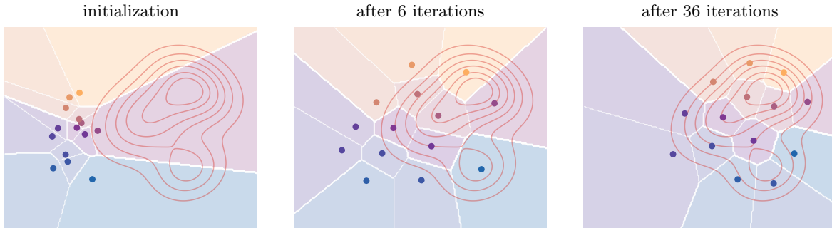
Figure 27: Lloyd quantization for the same continuous density and initial sites as Figure 26. The red contours show the density \alpha , while the colored disks are the current codepoints and have the same colors as their Voronoi cells. The iterations move the initially left-located sites toward the high-density region and reshape the cells according to centroidal Voronoi geometry.
