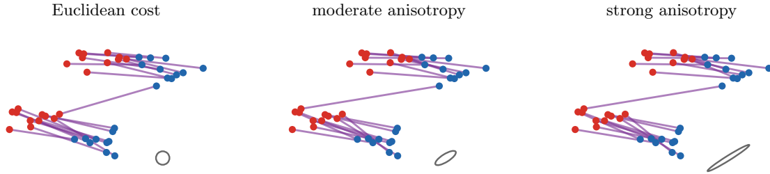
Figure 44: Changing the ground metric changes the optimal coupling. The same red and blue empirical measures are matched with c_A(x, y) = (x - y)^\top A(x - y) for the Euclidean metric and two increasingly anisotropic Mahalanobis metrics. The small gray ellipse shows the unit ball of the metric: directions in which the ellipse is elongated are cheaper, and this deforms the transport segments selected by the OT plan.
