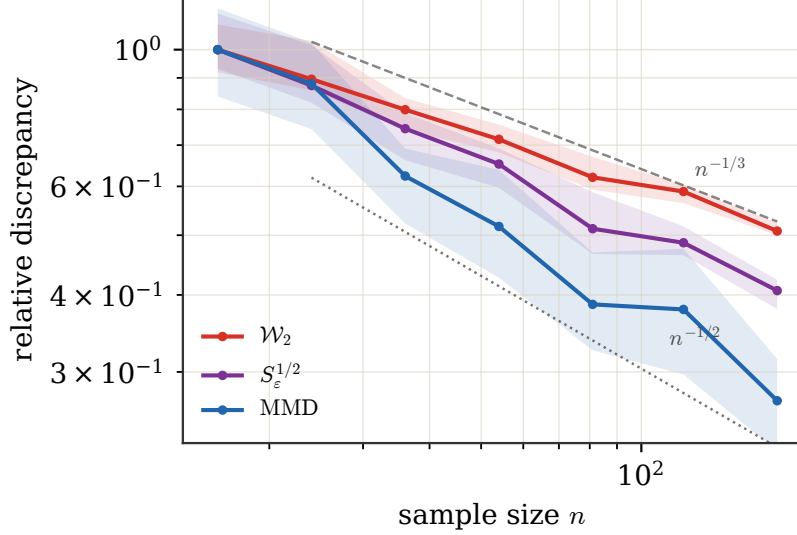
Figure 34: Empirical fluctuation in dimension three. For each sample size n , two independent empirical measures \alpha_n and \alpha'_n are drawn from the same standard Gaussian law in \mathbb{R}^3 . The curves show the median of D(\alpha_n, \alpha'_n) , normalized by its value at the smallest displayed n , with interquartile bands. Exact OT follows the slower dimension-dependent scale, while MMD and the fixed- \varepsilon Sinkhorn divergence behave closer to the parametric n^{-1/2} guide. This is a statistical illustration, not a solver benchmark.
