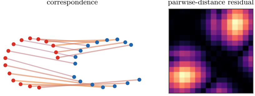
Figure 47: Local distortion in a non-isometric GW match. The left panel colors transport segments by the average residual induced by the displayed hard correspondence. The right panel shows the pairwise-distance residual matrix |d_{\mathcal{X}}(x_i, x_{i'}) - d_{\mathcal{Y}}(y_{\sigma(i)}, y_{\sigma(i')})| , which is the local contribution minimized by the discrete GW objective for this correspondence.
