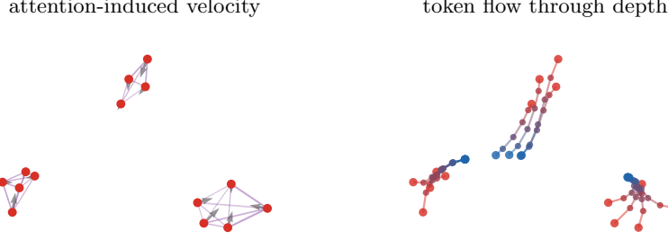
Figure 61: Attention as a transportation dynamics on token measures. The schematic uses the attractive setup Q = K = I and velocity W(X)X - X , where W(X) is the softmax attention matrix. The left panel shows one layer: faint violet edges encode attention weights and gray arrows show the residual velocity applied to red tokens. The right panel follows the same tokens through residual depth, colored from red to blue, and shows local clustering induced by attention.
