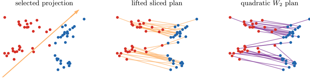
Figure 39: Lifted min-sliced plan. A one-dimensional direction is selected by a small deterministic sweep, then red and blue atoms are sorted after projection and matched in that order. The middle panel lifts this one-dimensional matching back to the plane; it is a feasible coupling but not the same object as the quadratic W_2 matching shown on the right. This illustrates why sliced constructions are computationally light and interpretable, while losing some of the geometry of the full transport problem.
