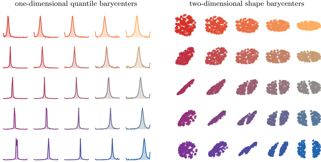
Figure 42: Wasserstein barycenter grids for four corner measures. The left panel uses the one-dimensional formula Q_{u,v} = \sum_{i,j} \lambda_{ij}(u,v) Q_{ij} and displays the densities reconstructed from the averaged quantiles. The right panel uses four deformation maps from a common reference cloud to simple shapes and averages these maps with the same bilinear weights, which is the discrete Monge analogue of a barycentric map. Colors interpolate between the four corners.
