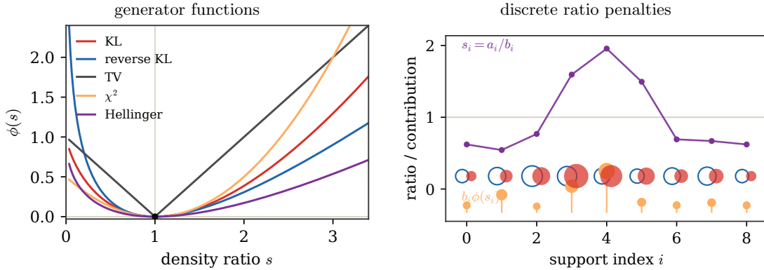
Figure 31: \varphi -divergences through density ratios. The left panel shows normalized generators for common divergences as functions of s = d\alpha/d\beta ; all curves vanish at s = 1 up to affine normalization. The right panel shows the discrete formula D_\varphi(a||b) = \sum_i b_i \varphi(a_i/b_i) : hollow blue circles encode b_i , filled red circles encode a_i , the violet curve gives the ratios a_i/b_i , and orange lollipops show local KL-type contributions.
