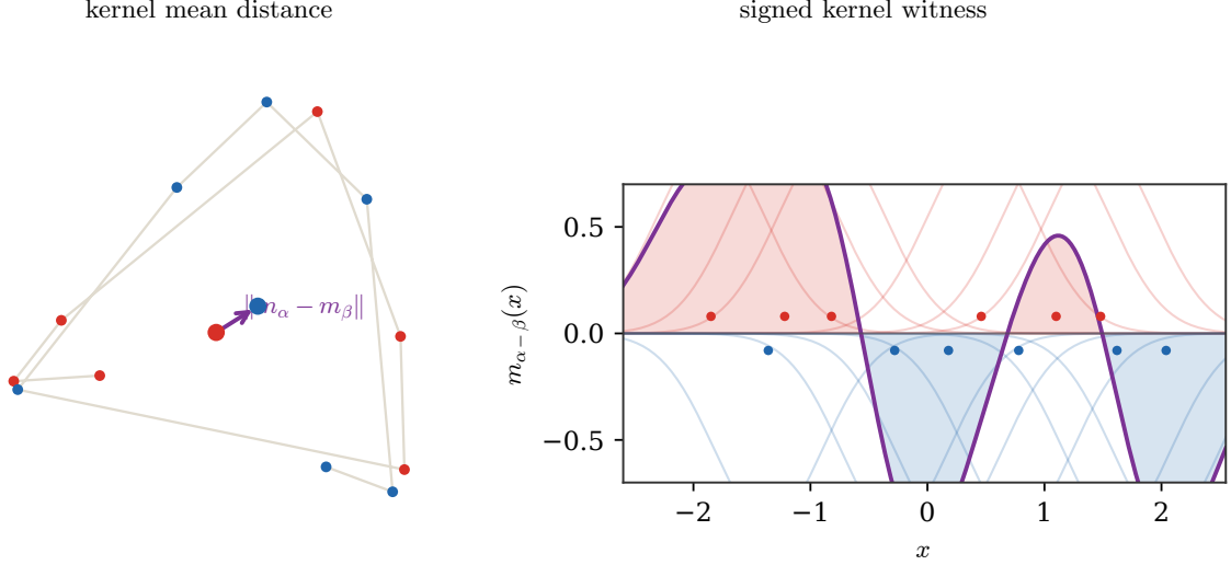
Figure 30: Kernel mean embedding interpretation of MMD. The left panel represents each distribution by its RKHS mean element m_\alpha or m_\beta , and the MMD is their Hilbert distance. The right panel shows the same difference in the input space: each Dirac contributes a kernel bump with its signed weight, and the optimal RKHS witness is proportional to m_\alpha - m_\beta .
