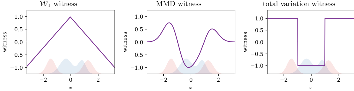
Figure 29: Dual witnesses for integral probability metrics. The red and blue curves are two one-dimensional probability densities and the violet curve is a representative normalized maximizer in the corresponding test class. \mathcal{W}_1 restricts the slope, MMD restricts the RKHS norm and produces a smooth witness, while total variation can saturate pointwise and therefore reacts sharply to signed density differences.
