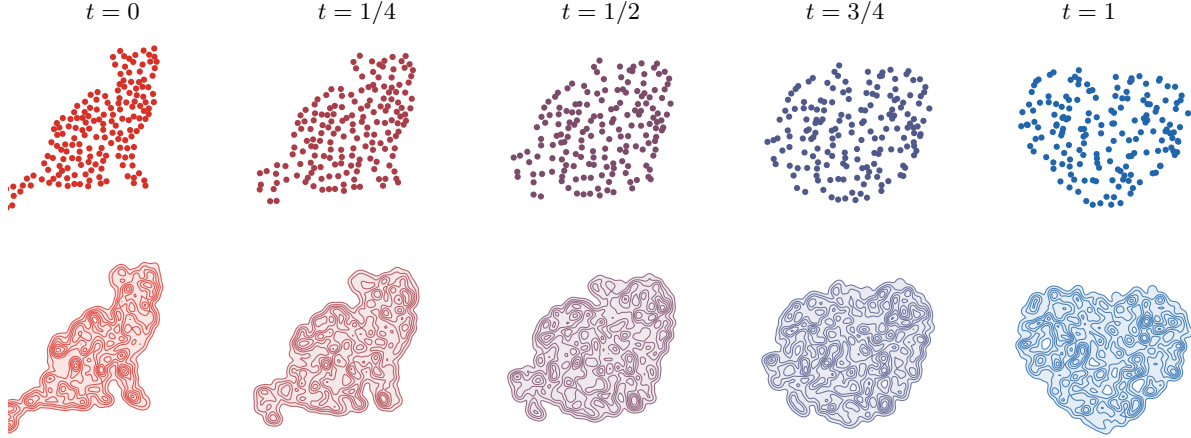
Figure 6: McCann displacement interpolation between a cat silhouette and a heart silhouette. The first row displays transported particles along T_t(x) = (1-t)x + tT(x) ; the second row shows kernel-smoothed densities computed from a larger cloud, making the evolving support easier to read.
