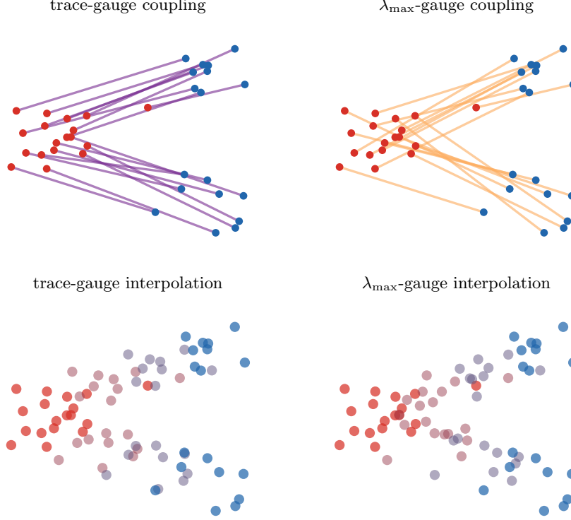
Figure 41: Trace and spectral gauges for displacement covariances. The trace gauge minimizes the average squared displacement and gives the usual quadratic transport plan. The \lambda_{\max} gauge penalizes the worst projected displacement variance; the displayed plan is obtained by a small finite-direction robust linear program. The bottom row shows the corresponding displacement interpolations, colored from red to blue. The figure is illustrative: it visualizes how changing the gauge changes the coupling and the induced interpolation geometry.
