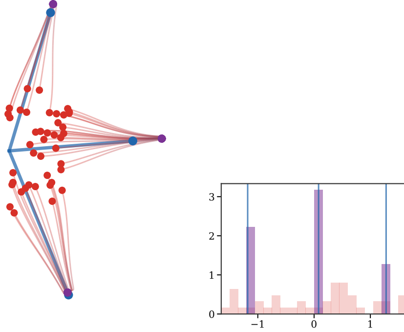
Figure 55: Mean-field training of a homogeneous two-layer model as transport in neuron space. Blue rays represent teacher directions or active homogeneous features. Red neurons move as particles under a Wasserstein gradient flow, rotating and changing radius until their empirical support concentrates near the useful rays. The right panel shows the same effect in angular coordinates: the initial red directional distribution becomes concentrated around the blue teacher rays. This illustrates why support propagation in parameter space is central to the homogeneous mean-field analysis.
