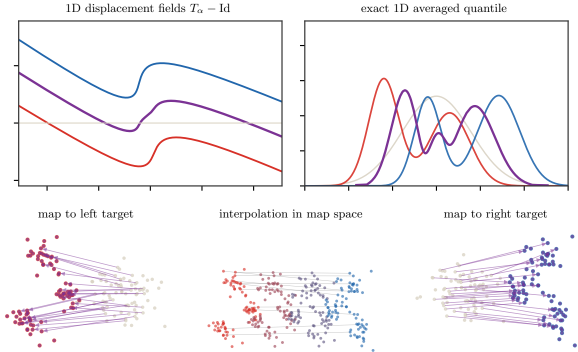
Figure 40: Linear OT coordinates. Fixing a reference measure \rho turns each target into the displacement field T_\alpha - \text{Id} . In one dimension this is exactly the quantile parametrization of \mathcal{W}_2 , so averaging displacement fields gives the true Wasserstein barycenter. In two dimensions the same construction averages Brenier maps from a central Gaussian reference toward two multimodal targets; it is a tangent approximation and should not be confused with the generally nonlinear Wasserstein barycenter.
