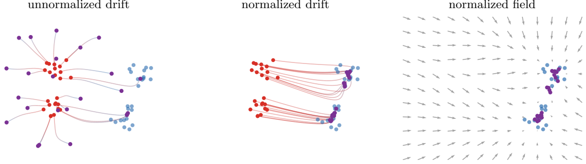
Figure 60: Drifting fields for a small particle generator. The unnormalized Laplacian-kernel drift has weak long-range attraction and can leave particles away from the data modes. The normalized drift uses the local average B_\varepsilon[\beta] - B_\varepsilon[\mu_t] , so particles reach the blue modes while the self-normalized correction prevents collapse. The right panel displays the normalized vector field around an intermediate violet model distribution.
