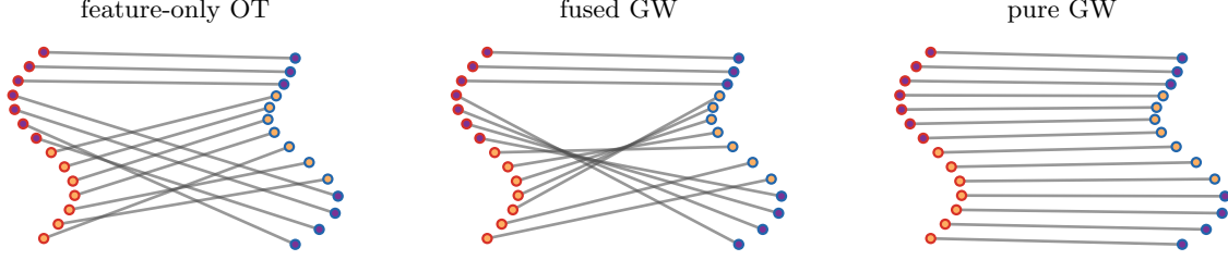
Figure 48: Feature information and intrinsic geometry in fused Gromov–Wasserstein. Small inner disks encode binary node features. Feature-only OT follows the attributes even when this crosses the shape structure, pure GW follows the intrinsic ordering, and fused GW balances the feature term with the pairwise-distance distortion.
