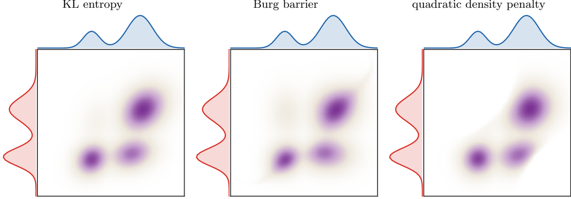
Figure 35: Effect of the density-ratio regularizer on the coupling. The red and blue side curves are fixed one-dimensional Gaussian-mixture marginals. The central matrix displays the square root of the coupling density on a common color scale. KL regularization gives the usual diffuse positive plan, the Burg barrier keeps a positive but differently tailed support, and the quadratic density penalty can set entries exactly to zero through its positive-part law.
