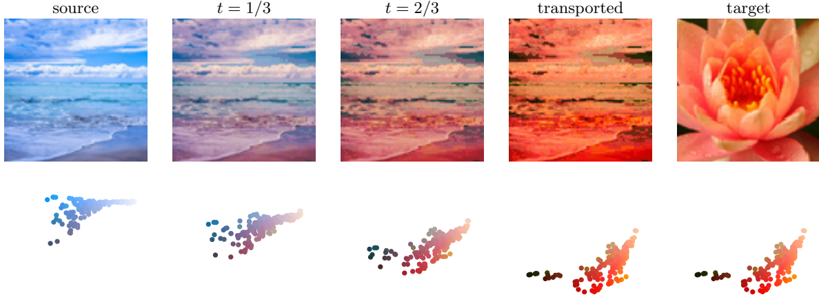
Figure 5: Color transfer as a Monge map in RGB space, from a beach photograph to a flower photograph. The top row applies the palette map to the source image; the bottom row shows the empirical color clouds in the RGB cube. Only colors are transported here, not pixel locations.
