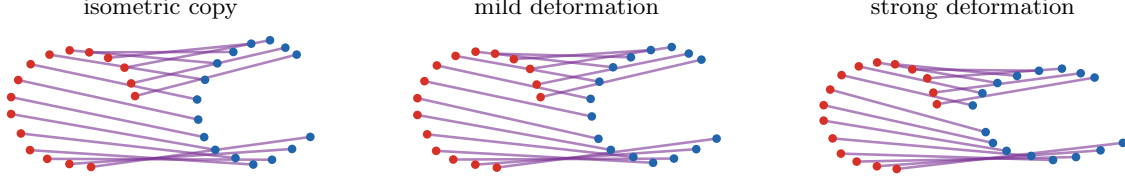
Figure 46: Gromov–Wasserstein correspondences under increasing deformation. The red and blue point clouds are not compared through an ambient Euclidean cross-cost; instead, the GW coupling compares their internal pairwise distances. A perfectly isometric copy admits a clean structural match, while mild and strong deformations progressively bend the correspondence.
