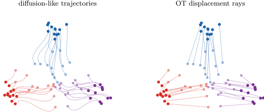
Figure 59: Diffusion-style sampling trajectories compared with OT rays in a small two-dimensional example. The initial particles are sampled near the center and each trajectory is colored, including its initial disk, by the final target cluster. Curved multi-step trajectories can approach modes through non-straight paths, while the OT map uses straight displacement rays selected by the quadratic matching.
