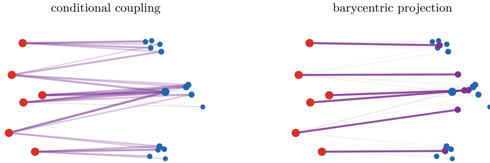
Figure 45: Weak barycentric transport on a small discrete coupling. The left panel shows the full conditional laws: each red source atom splits its mass among several blue target atoms, with segment thickness proportional to transported mass. The right panel collapses each conditional law \pi_x to its barycenter \bar{y}(x) = \int y d\pi_x(y) , shown in violet. The barycentric weak cost only sees the red-to-violet displacement, and therefore ignores the conditional spread around each barycenter.
