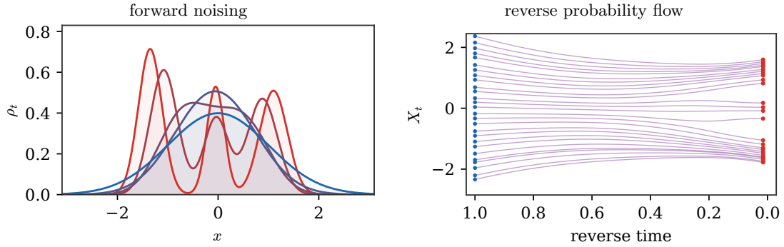
Figure 57: One-dimensional diffusion bridge for a Gaussian-mixture data law. The forward path Z_t = (1-t)X + tY smooths the red data density toward a blue Gaussian endpoint. Reversing the probability-flow ODE transports a denser set of blue noise samples back toward the data modes, making the splitting of trajectories across mixture components visible.
