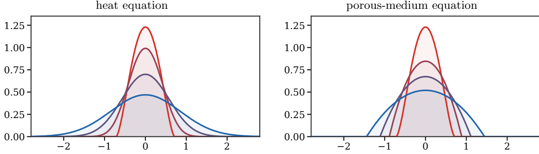
Figure 52: Two entropy-driven Wasserstein gradient flows from the same compact initial density. The heat flow is generated by Shannon entropy g(\rho) = \rho \log \rho and instantly develops Gaussian tails. The porous-medium flow uses the power entropy g(\rho) = \rho^m / (m - 1) with m = 2 , hence \partial_t \rho = \Delta(\rho^2) ; it spreads more slowly and keeps a compact free boundary.
