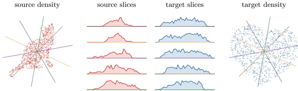
Figure 38: Sliced Wasserstein projections between two planar densities. Five fixed directions are drawn on the source and target point clouds. For each direction, the middle panels show the one-dimensional projected histograms (P_\theta)_\# \alpha and (P_\theta)_\# \beta . Sliced OT averages one-dimensional Wasserstein discrepancies over many such directions, replacing a difficult planar comparison by a collection of sorted one-dimensional comparisons.
