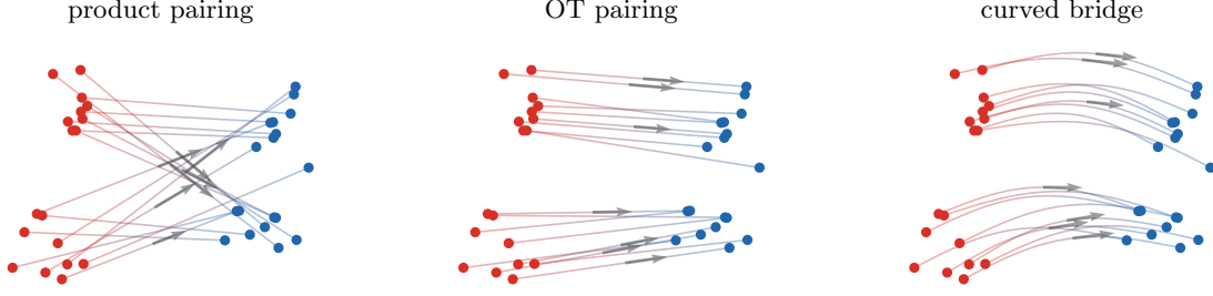
Figure 56: Flow matching interpolants between the same empirical source and target measures. A product-style random pairing produces crossing paths, an OT pairing gives direct displacement rays, and a curved bridge changes the path geometry while keeping the same endpoints. Gray arrows mark representative midpoint velocities \partial_t P_t .
