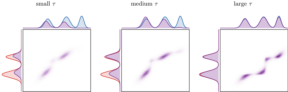
Figure 36: KL unbalanced OT on one-dimensional Gaussian-mixture densities. The central matrix is the transported coupling. On the left, the red curve is the prescribed source marginal and the violet curve is the transported source marginal; the red gap is destroyed mass. On the top, the blue curve is the prescribed target marginal and the violet curve is the transported target marginal; the blue gap is created mass. Increasing \tau makes marginal mismatch more expensive, so more mass is transported, including toward the far right target mode.
