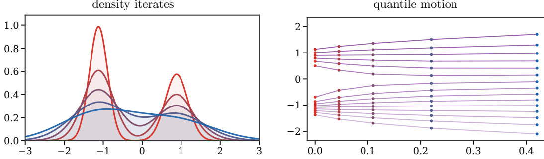
Figure 51: JKO minimizing movements for the entropy flow in one dimension. The left panel displays successive implicit-Euler minimizers for the heat equation, colored from red to blue. The right panel tracks inverse CDF values Q_t(s) = F_t^{-1}(s) for selected probability levels s , giving a Lagrangian view of the proximal movement in Wasserstein space.
