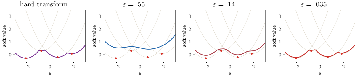
Figure 32: Soft c -transforms for decreasing temperatures. The hard transform is the lower envelope of shifted cost functions, while a positive \varepsilon replaces the pointwise minimum by a log-sum-exp soft minimum. As \varepsilon decreases, the soft transform sharpens and approaches the non-smooth hard envelope.
