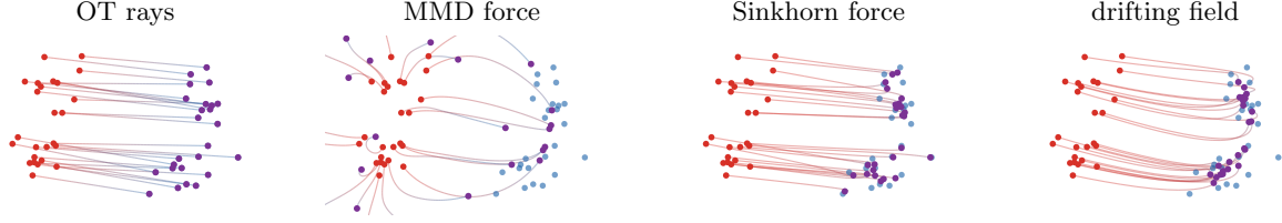
Figure 54: Particle trajectories induced by different discrepancy geometries. The red particles and blue target cloud are the same in all panels. Straight OT displacement produces rays from an optimal matching; an MMD-type witness field gives smoother nonlocal forces; the Sinkhorn-divergence force is an entropic, debiased transport attraction; and the normalized drifting field combines attraction to data with self-repulsion. The figure is qualitative: it compares geometric behavior, not solver performance.
