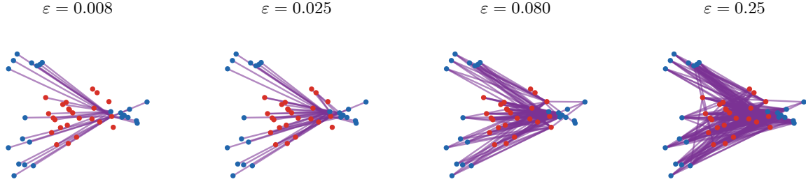
Figure 21: Entropically regularized couplings between the canonical red and blue point clouds for four fixed regularization strengths. The squared Euclidean cost is normalized by its median. Violet segments display the largest visible entries of the computed Sinkhorn plan, with thickness and opacity proportional to transported mass. The computed plans are strictly positive for every \varepsilon > 0 , but the visible mass pattern evolves from nearly sparse to diffuse as \varepsilon increases.
