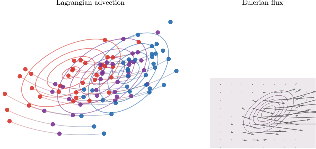
Figure 49: Two views of the continuity equation. The left panel advects particles and Gaussian density contours under a smooth affine vector field, showing the Lagrangian flow x'(t) = v(x(t)) . The right panel shows the Eulerian flux m_t = \rho_t v_t at an intermediate time, where \alpha_t = \rho_t dx : arrows are weighted by the local density, so the velocity contributes to the PDE only where mass is present.
