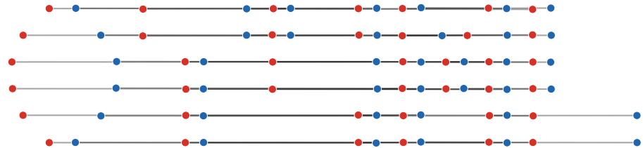
vertical rank one, A = -e_2 e_2^\top
