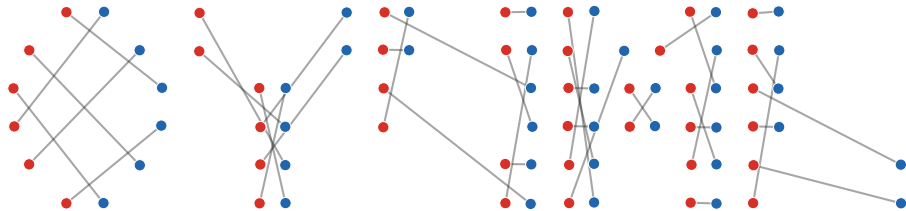
horizontal rank one, A = -e_1 e_1^\top
