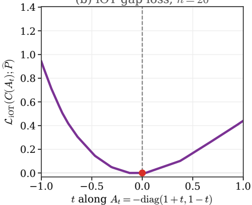
(b) iOT gap loss, n = 20
