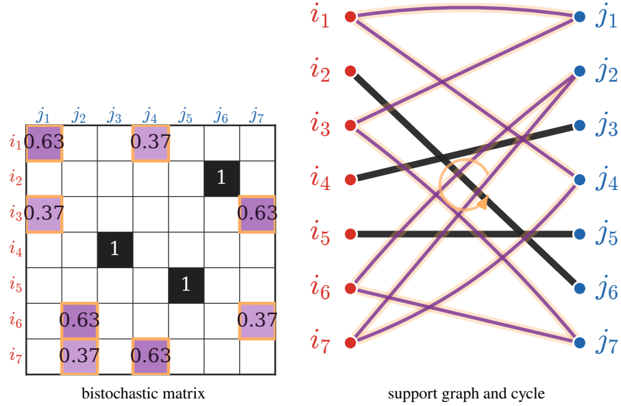
Figure 1.8: Cycle certificate in the Birkhoff–von Neumann proof. The matrix is bistochastic but not a permutation matrix. Its positive support defines a bipartite graph; a fractional cycle permits an alternating add-subtract perturbation that preserves row and column sums and pushes at least one entry to zero. Repeating this exposes permutation matrices as extreme points.
