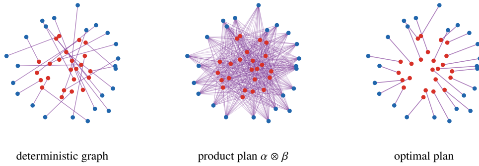
Figure 1.7: Discrete couplings represented as straight transport segments. A deterministic graph coupling sends each source to one destination, the product plan spreads every source mass over all targets, and the optimal Kantorovich plan minimizes the quadratic cost while being allowed to split mass. Line width and opacity encode the transported mass.
