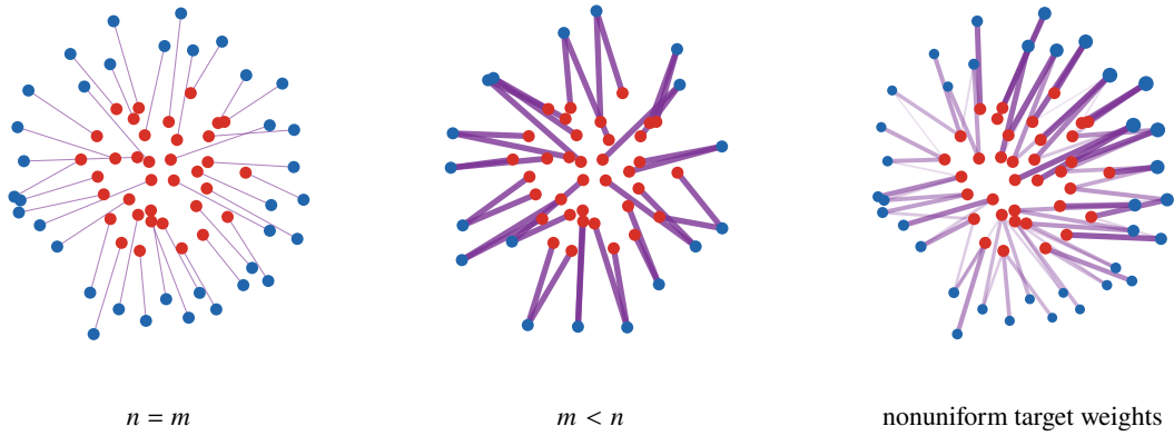
Figure 1.11: From assignments to transport plans, using the same disk-to-annulus geometry as Figure 1.6. In the balanced equal-weight case, each source atom is matched to one target atom. With fewer target atoms, or with strongly nonuniform target weights, the coupling must merge or split mass; segment thickness and opacity encode transported mass.
