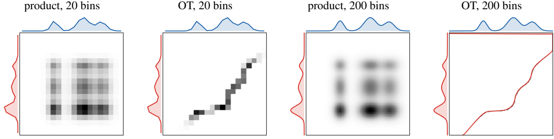
Figure 1.10: Coupling matrices with their prescribed marginals. The central grayscale image displays P_{ij} ; the red curve on the left is the source marginal a , and the blue curve on top is the target marginal b . The independent product plan is diffuse, whereas the one-dimensional optimal plan concentrates near the monotone quantile correspondence.
