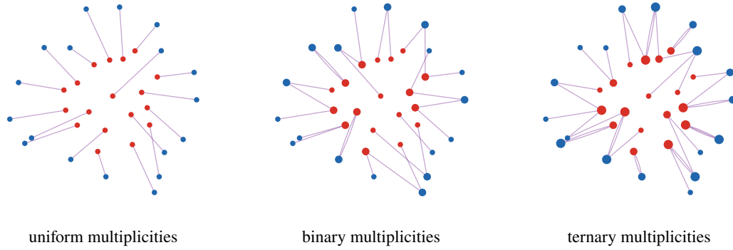
Figure 1.12: Rational weights as duplicated uniform matchings. The red and blue locations are displayed once, while disk areas encode integer multiplicities. After duplication, the uniform assignment may contain several matched copies of the same displayed point; collapsing these copies gives the integer count matrix underlying a rational-weight Kantorovich plan.
