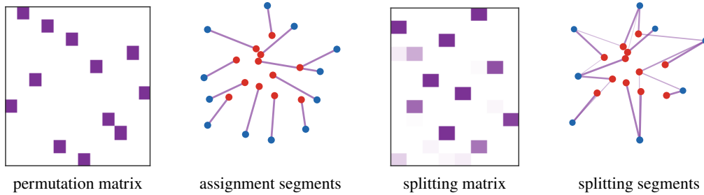
Figure 1.9: From permutation matrices to splitting couplings. When two empirical measures have the same number of atoms and uniform weights, an optimal plan can be a permutation matrix. Once target masses are nonuniform, admissible couplings may split one source among several targets or merge several sources into one target.
