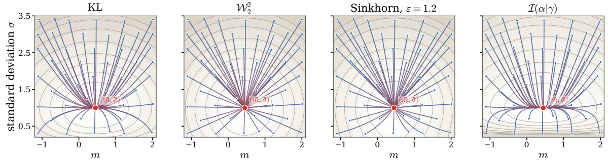
Figure 4.12: One-dimensional Gaussian Wasserstein gradient flows in the parameter half-plane (m, \sigma) . From left to right: relative entropy, squared Wasserstein distance, debiased Sinkhorn divergence, and relative Fisher information. The trajectories start from the same well-spread initial parameters and converge to the common target (\bar{m}, \bar{\sigma}) .
