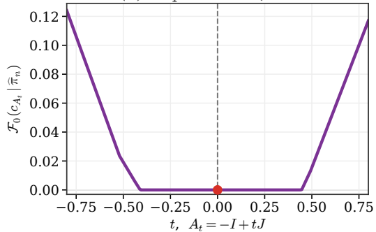
(b) empirical loss, n = 10
