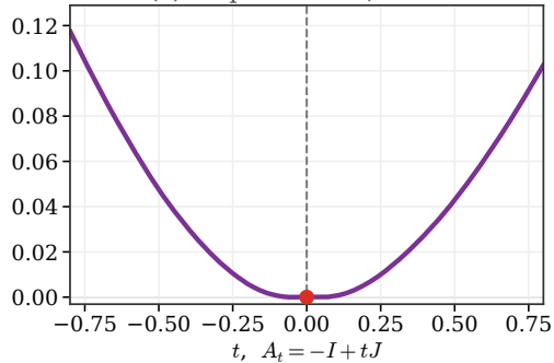
(c) empirical loss, n = 200
