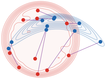
(a) samples from \pi_0
