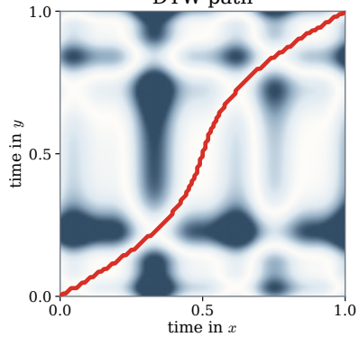
DTW path
