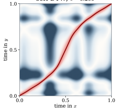
soft-DTW, \epsilon = 0.200
