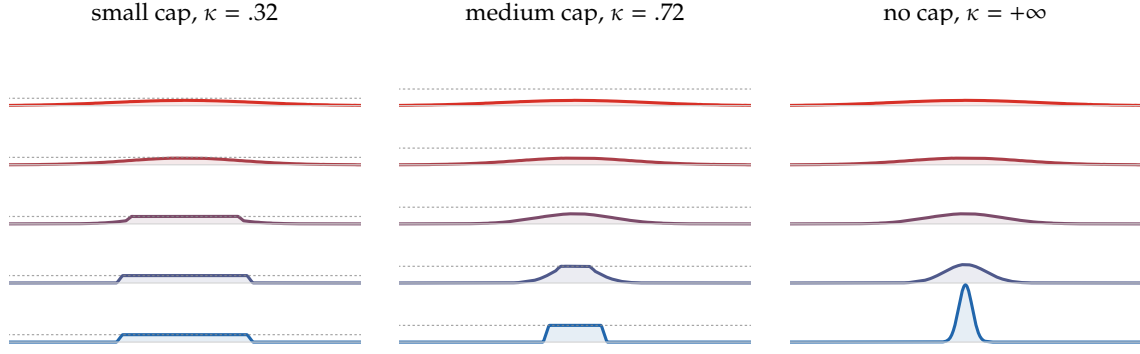
Figure 3.8: Density-constrained gradient flow under a quadratic attraction. The one-dimensional flow is computed in quantile variables by explicit Lagrangian descent followed by the isotonic projection enforcing \partial_s q \geq 1/\kappa . Each panel stacks five times vertically, colored from red to blue, using the same vertical density scale in all three panels. The dashed gray line marks the maximal density \kappa for the constrained runs. A small cap forces the mass to form a wide saturated block, a medium cap allows a narrower congested region, and the unconstrained flow concentrates freely near the minimizer of h .
