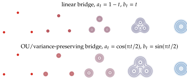
Figure 4.3: Two-dimensional noising paths from three Dirac masses to a single Gaussian. The top row shows the linear interpolation Z_t = (1-t)X + tY , whose component centers move linearly toward the origin and whose covariance grows like (t\sigma)^2 \text{Id} . The bottom row uses the variance-preserving Ornstein–Uhlenbeck coefficients a_\tau = e^{-\tau} and b_\tau = \sqrt{1 - e^{-2\tau}} , reparametrized by \tau = -\log \cos(\pi t/2) so that a_t = \cos(\pi t/2) and b_t = \sin(\pi t/2) . It has the same endpoints but a different speed of contraction and noising.
