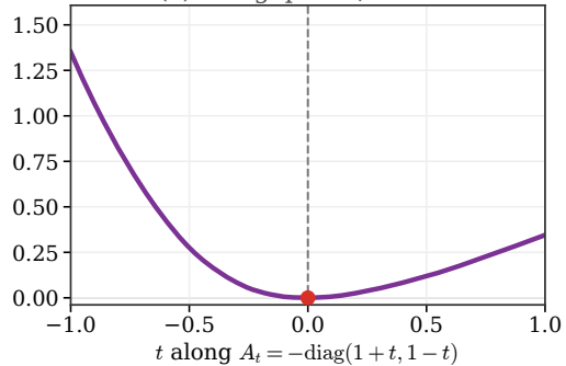
(c) iOT gap loss, n = 100
