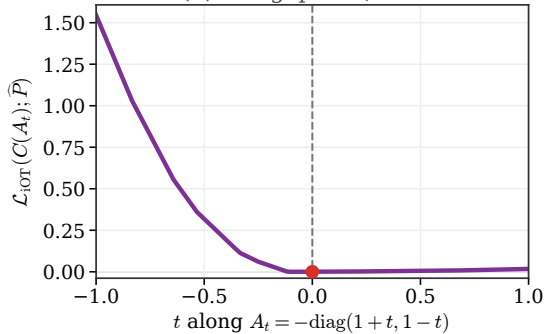
(b) iOT gap loss, n = 10
