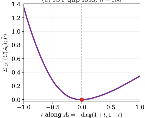
(c) iOT gap loss, n = 100
