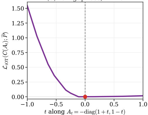
(b) iOT gap loss, n = 10
