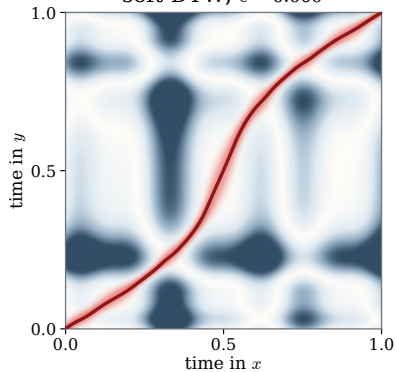
soft-DTW, \epsilon = 0.060
