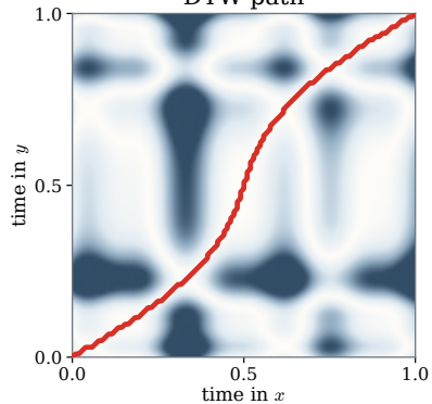
DTW path
