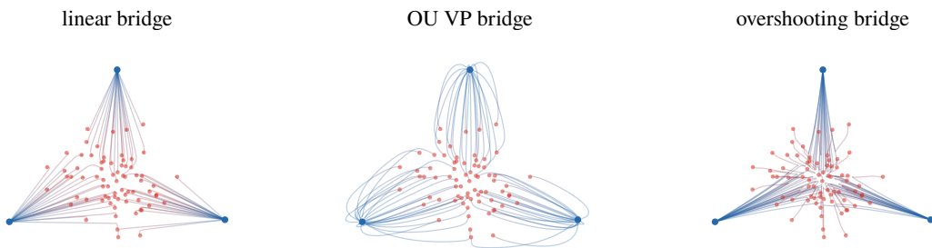
Figure 4.5: Effect of the interpolant on exact reverse-flow trajectories. All panels use the same three-Dirac target and the same Gaussian endpoint. The linear bridge a_t = 1 - t , b_t = t produces almost radial curves. The variance-preserving OU bridge a_\tau = e^{-\tau} , b_\tau = \sqrt{1 - e^{-2\tau}} changes the relative speed of contraction and noising. The overshooting bridge a_t = (1 - t)(1 - 2t) , b_t = t is not a time reparameterization of either one and produces a more pronounced bending of the reverse trajectories.
