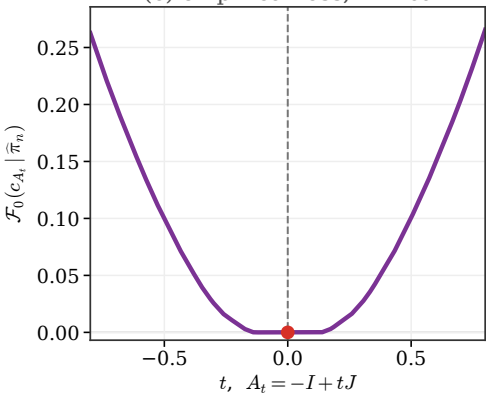
(c) empirical loss, n = 100
