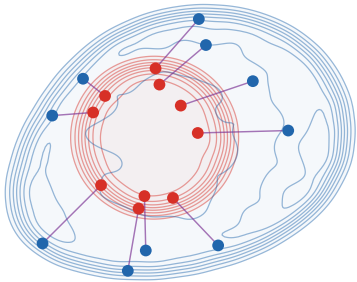
(a) samples from \pi_0
