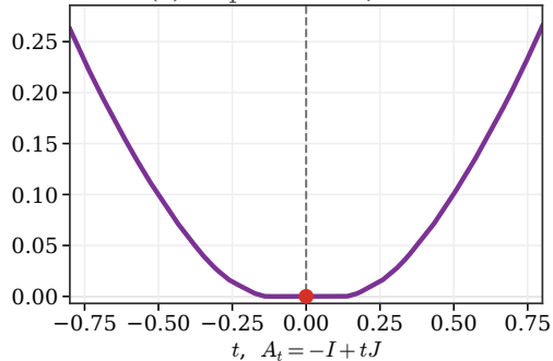
(c) empirical loss, n = 100
