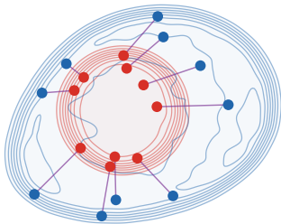
(a) samples from \pi_0
