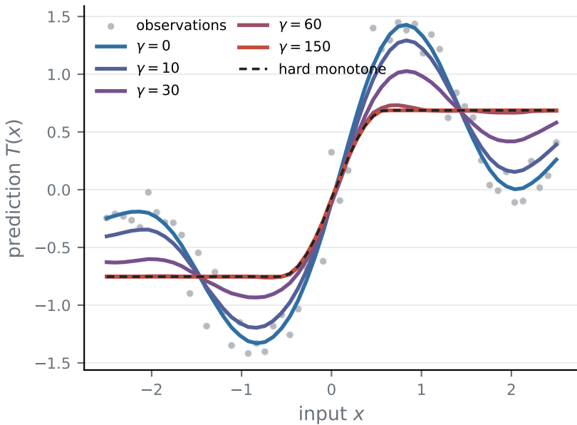
Kernel regression path
