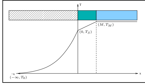
Figure 17.3: Temperature profile during solidification
