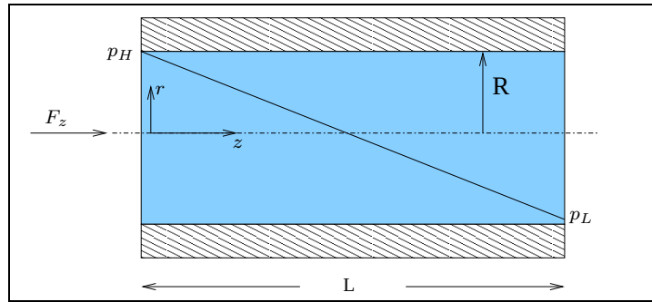
Figure 12.1: Pipe Flow
