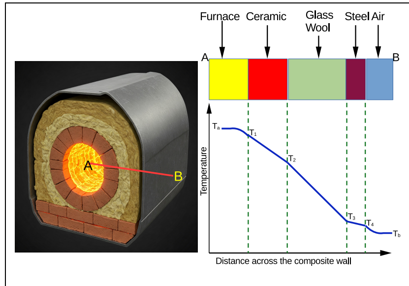
Figure 16.6: Schematic thermal profile across a composite wall of a furnace. The image of the furnace was created using Gemini 2.0 Flash.
