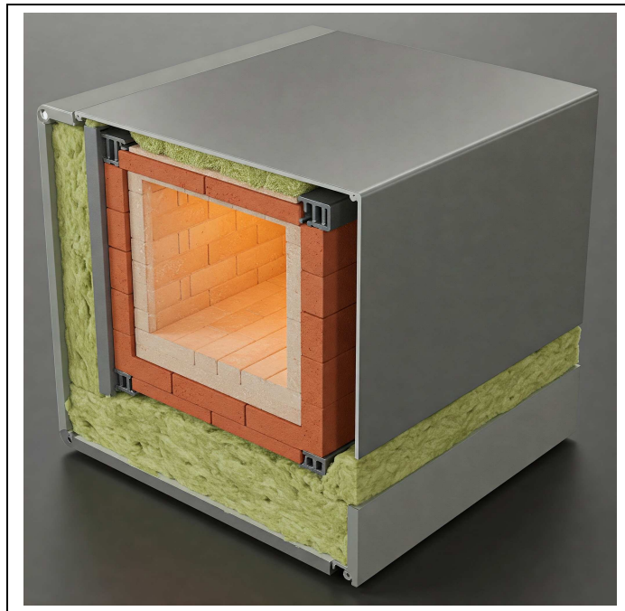
Figure 16.5: Box type multi-walled furnace schematic created using Gemini 2.0 Flash.
