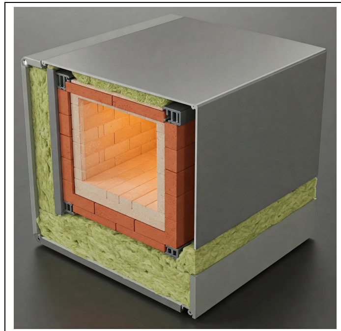
Figure 16.5: Box type multi-walled furnace schematic created using Gemini 2.0 Flash.
