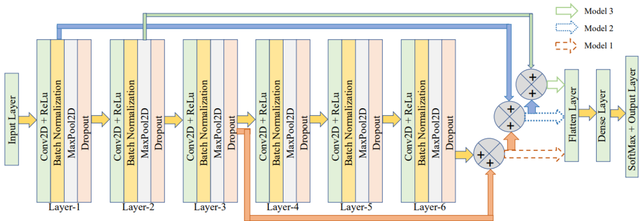
FIGURE 1: The architecture of the proposed classification method consists of three models shown in the architecture.
