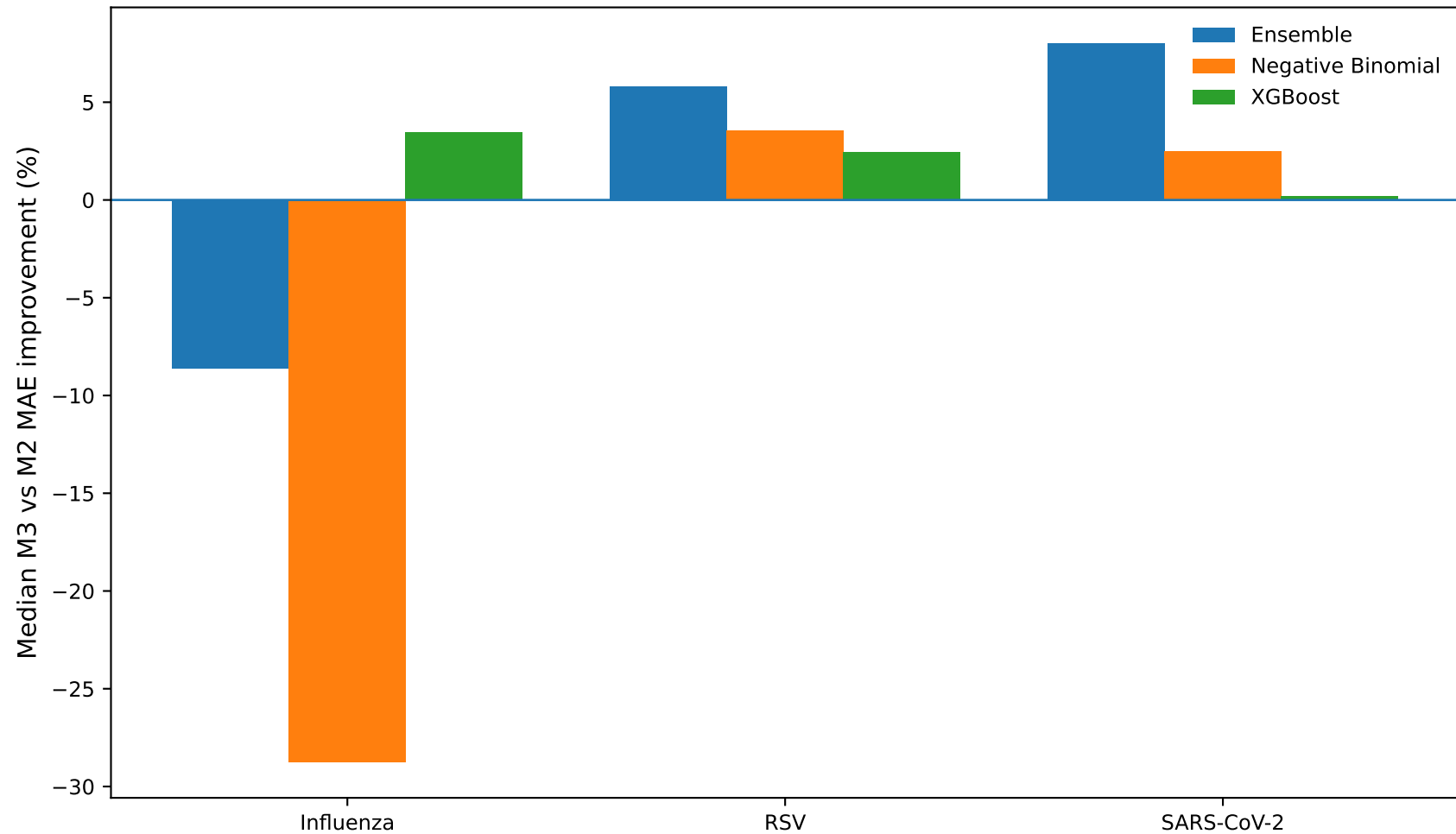
Effect of cross-pathogen information by target pathogen
