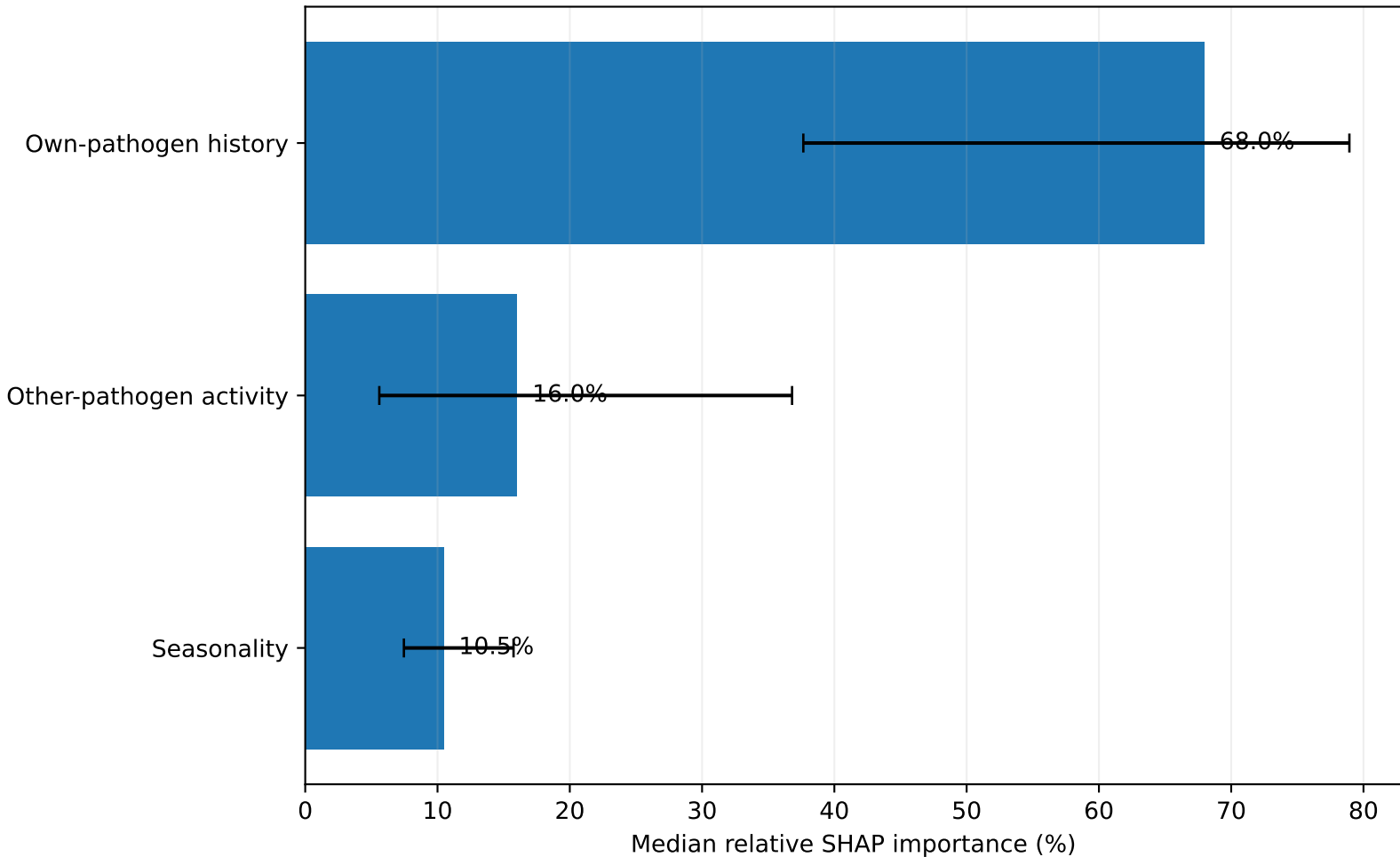
Relative contribution of predictor groups in XGBoost forecasts
