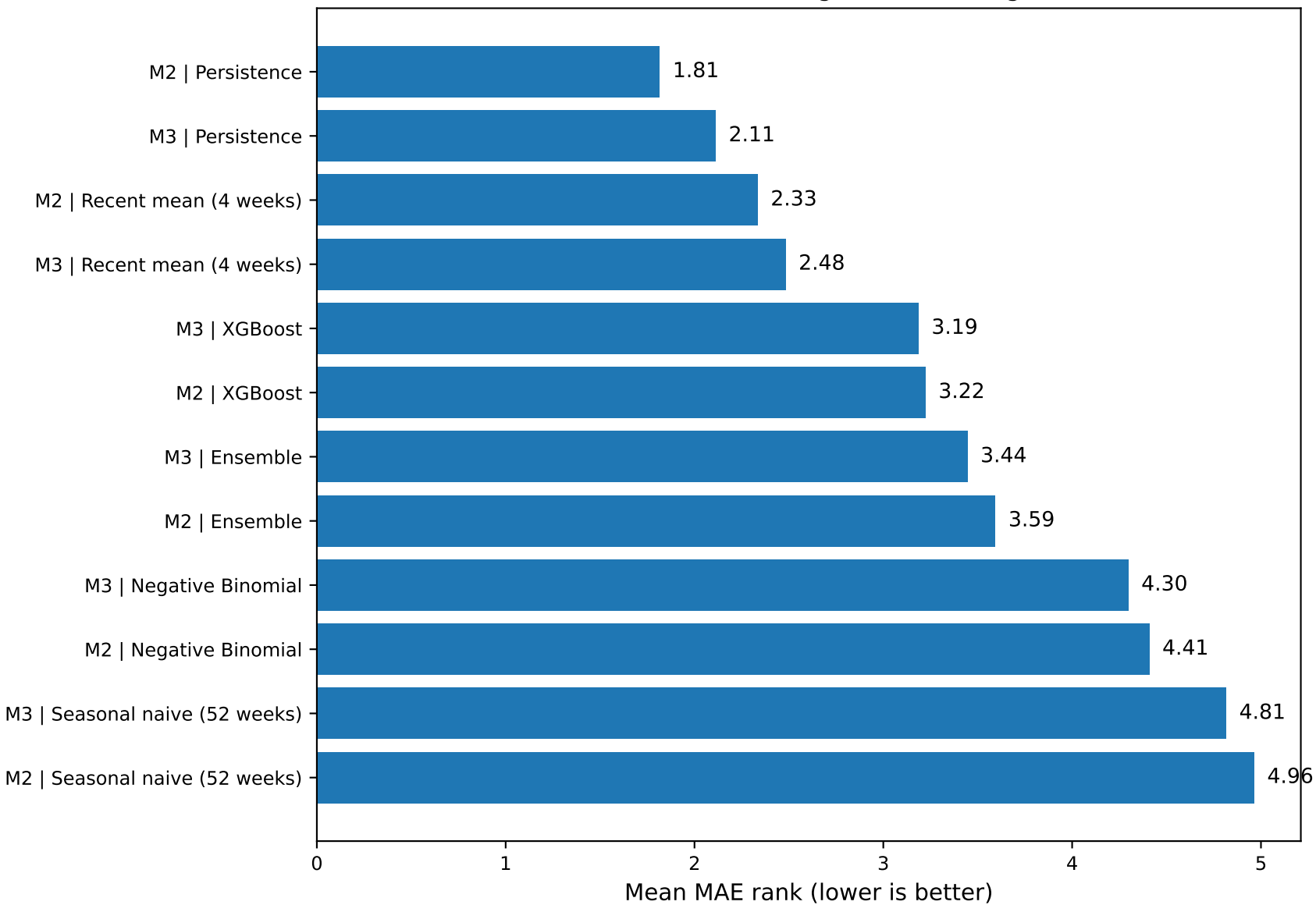
Overall forecasting model ranking
