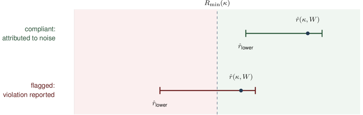
FIGURE 11. The reliability hypothesis test on a single number line.
