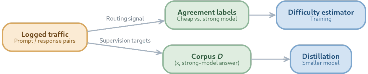
FIGURE 14. The training pipeline built from one logged dataset.
