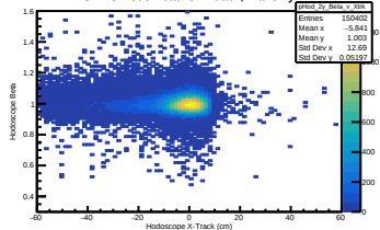
SHMS Hodo Beta vs. X-track, Plane 2y
